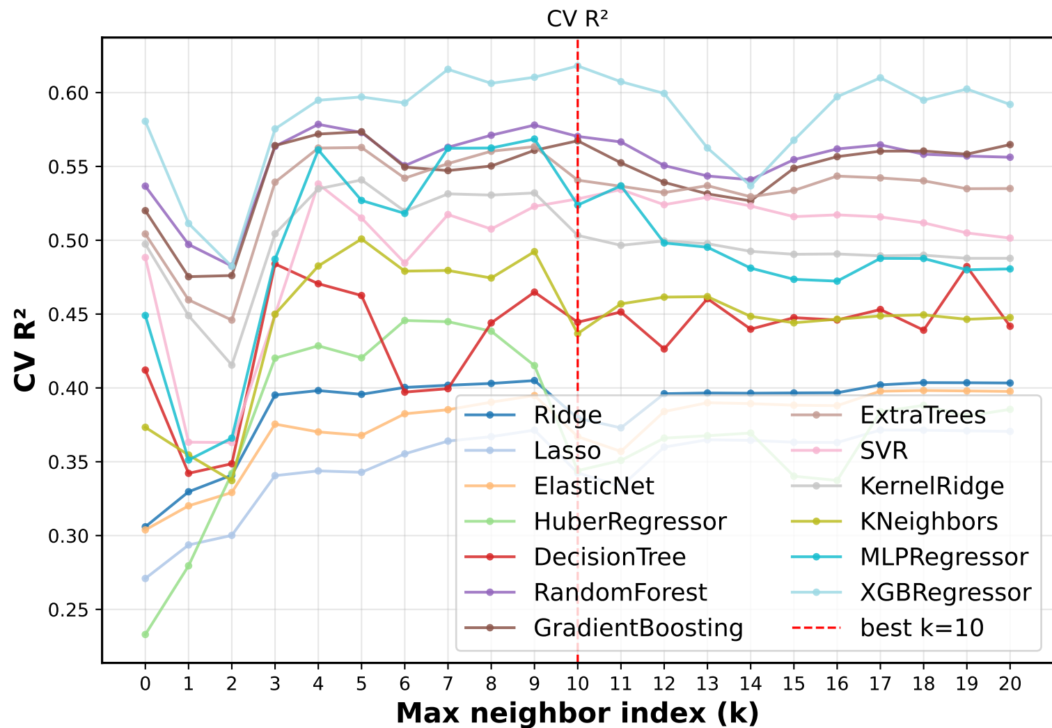
Neighbor Sweep — 5-Fold CV Performance on Training Set
