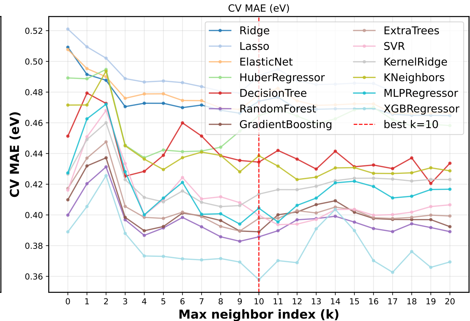
Neighbor Sweep — 5-Fold CV Performance on Training Set
