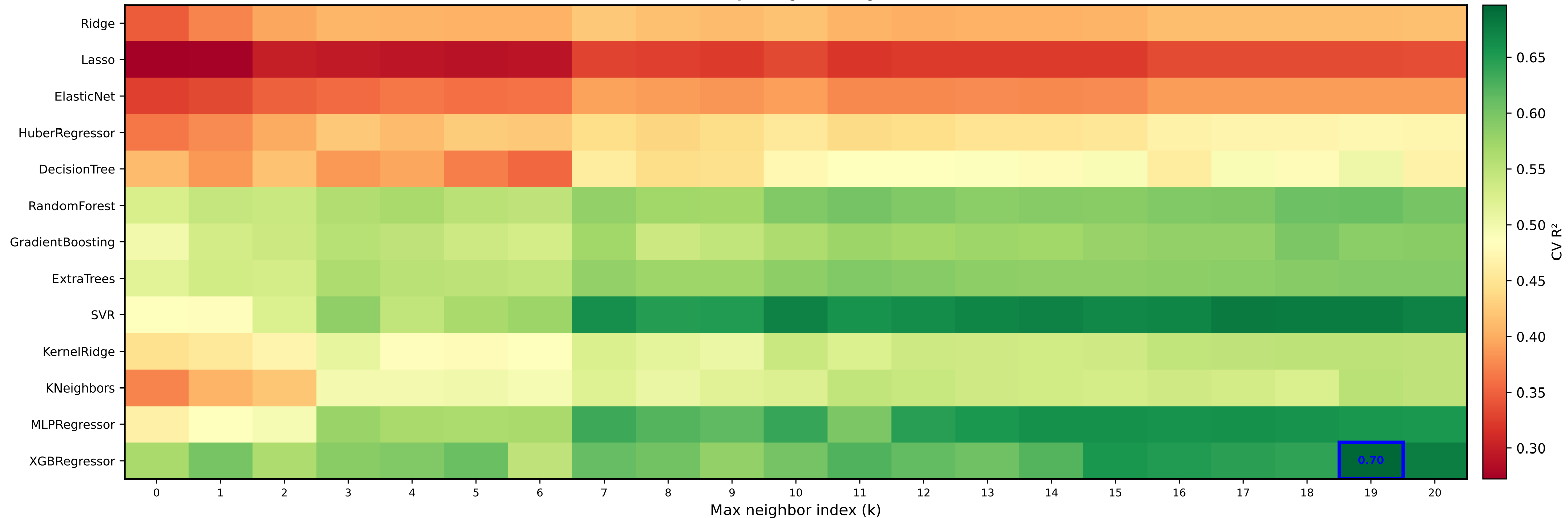
CV R 2 Heatmap — all models × all neighbor levels (red = poor, green = good)
