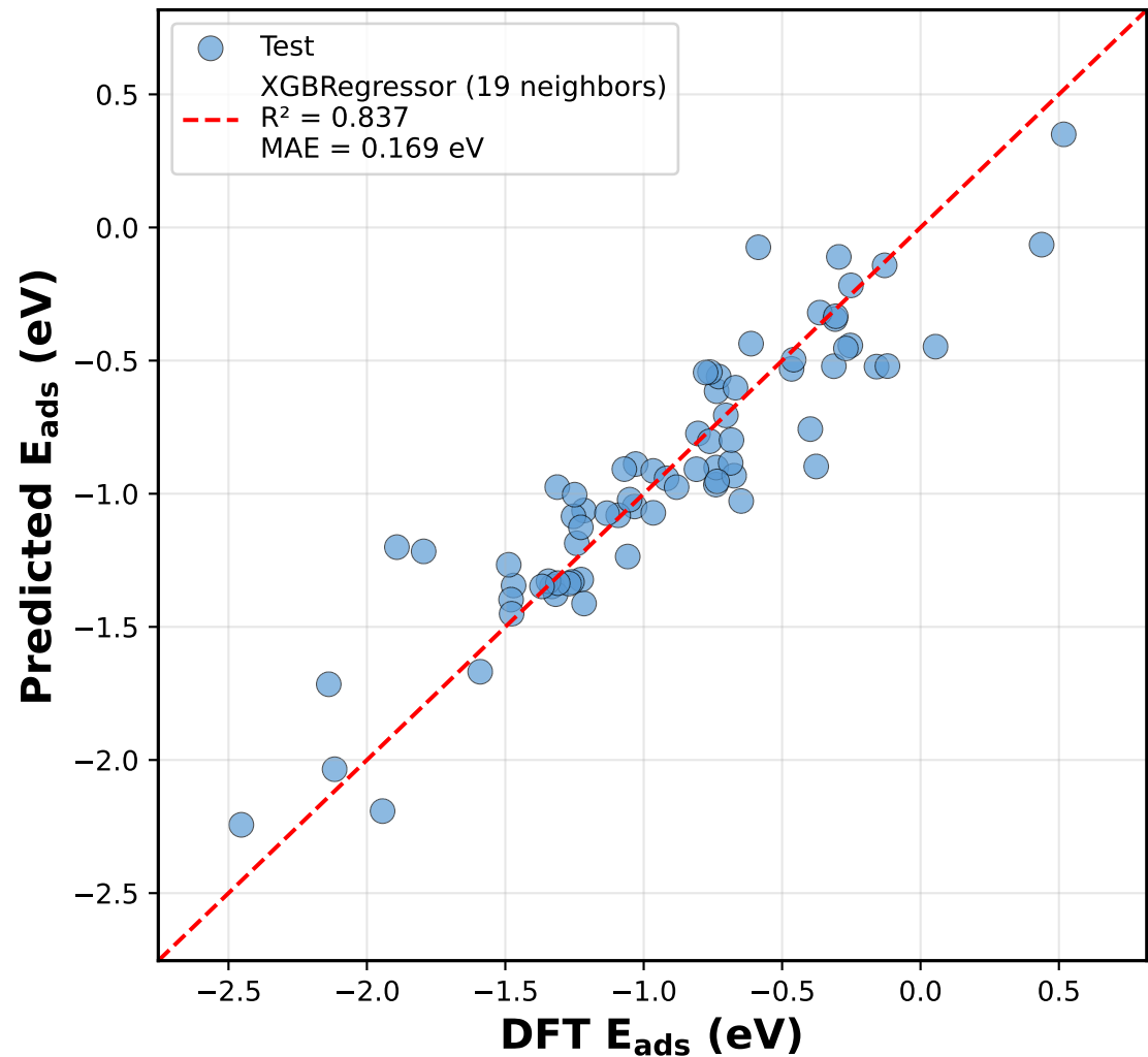
Parity Plot — XGBRegressor (neighbors 0..19) R^2=0.837 MAE=0.169 RMSE=0.229 eV
