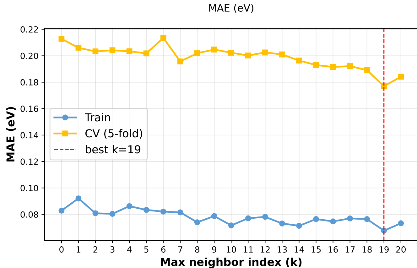
Train vs CV — XGBRegressor (best model)
