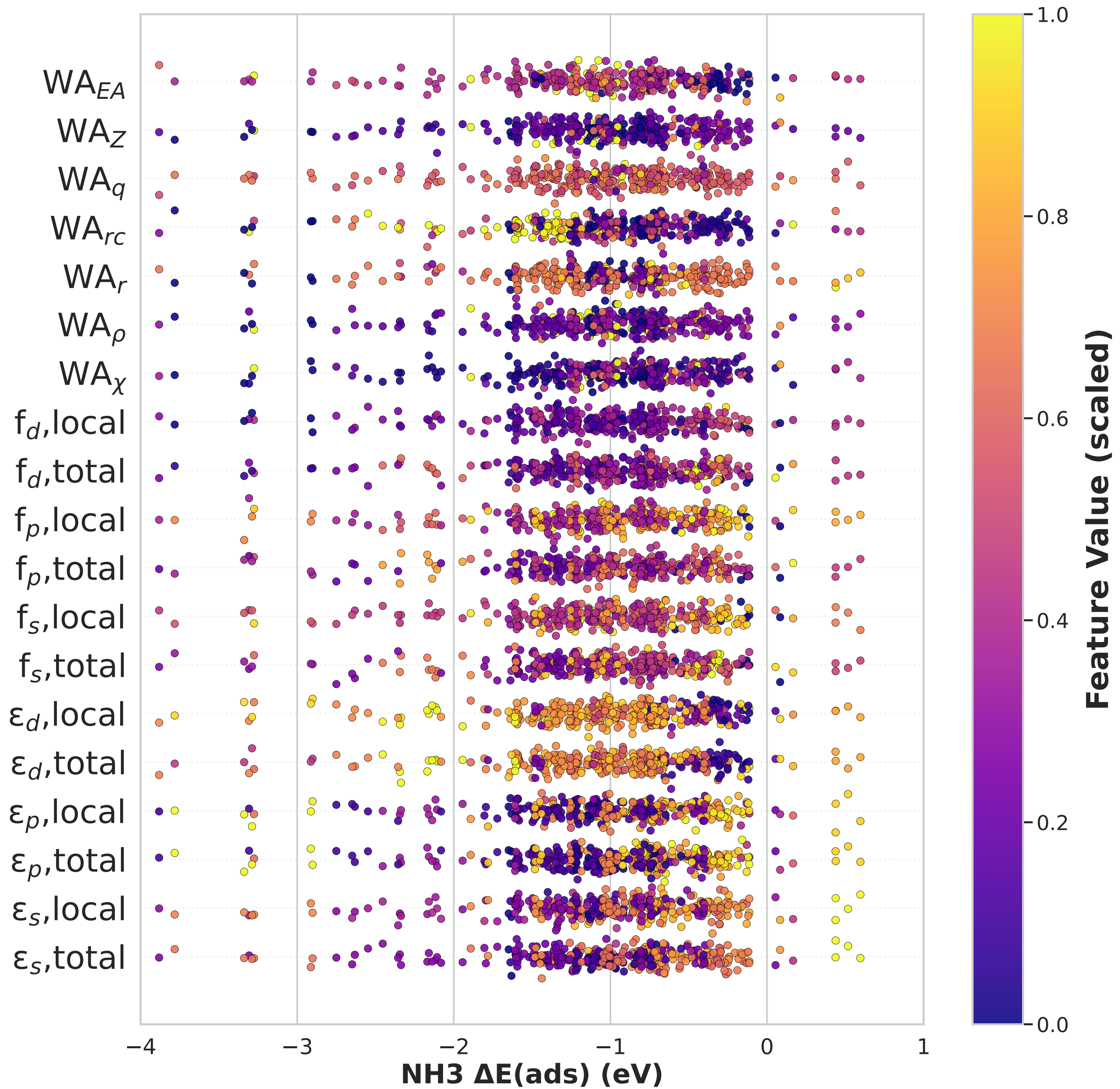
Feature-wise Adsorption Distribution (n = 3, NH3)
