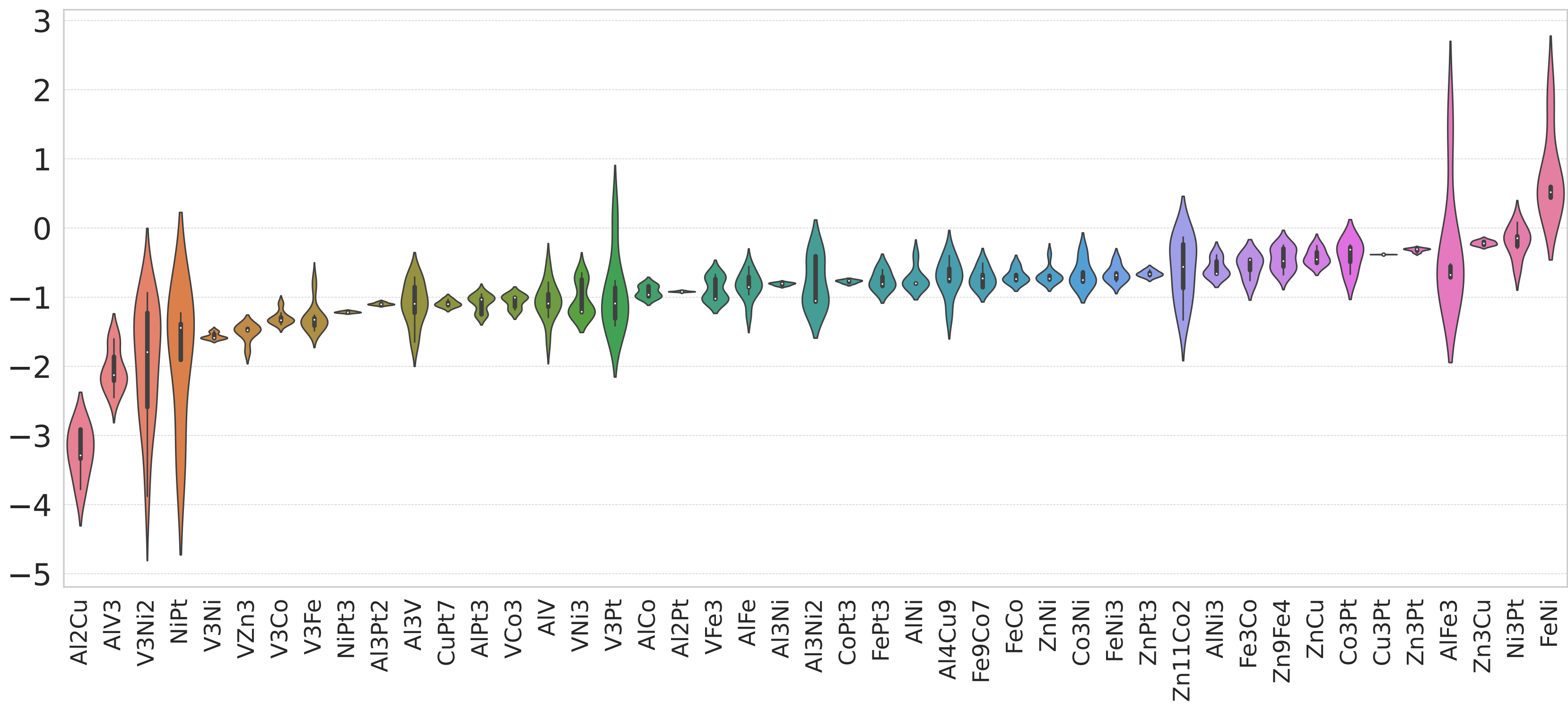
NH 3 \Delta E(\text{ads}) (eV)
