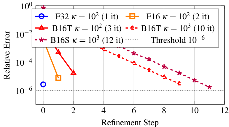
Figure 3: Iterative refinement convergence curves (n=256, seed=0). Solid lines show \kappa = 10^2 ; dashed lines show \kappa = 10^3 . F32 converges within factorization; F16 requires 2 iterations; B16T requires 3 iterations at low \kappa but 10 at high \kappa ; B16S requires up to 12 iterations. Convergence criterion: relative error < 10^{-6} (dotted).
