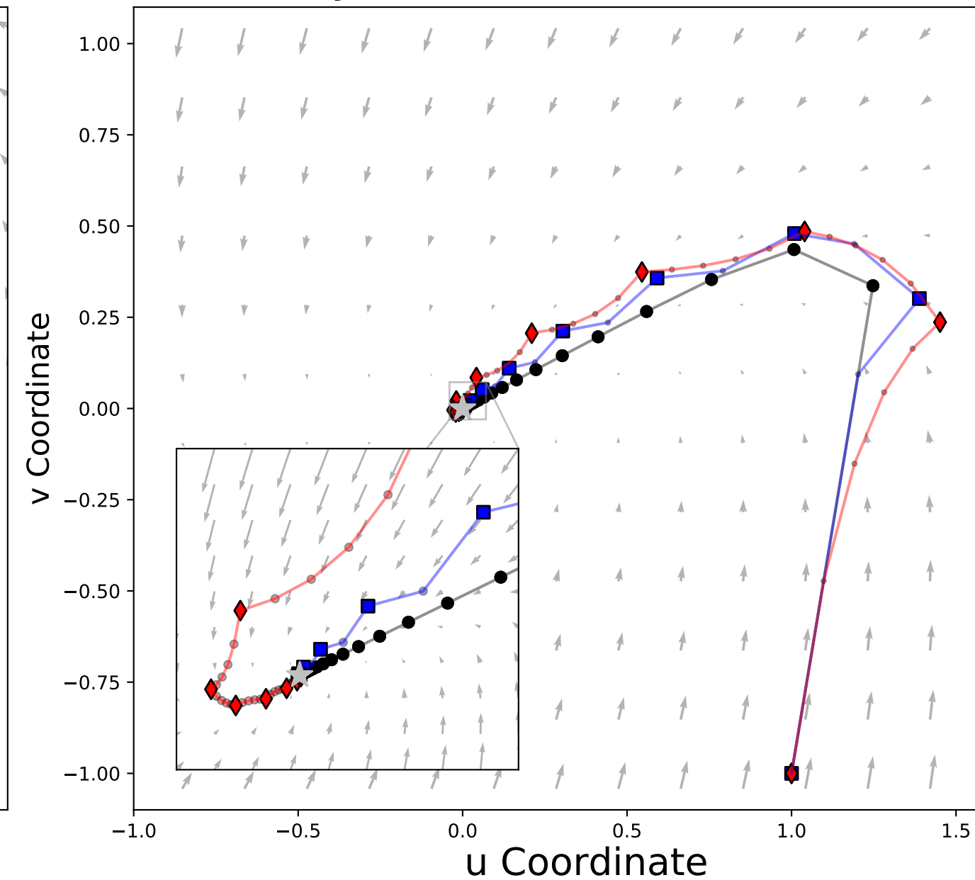
Trajectories for C=3.5
