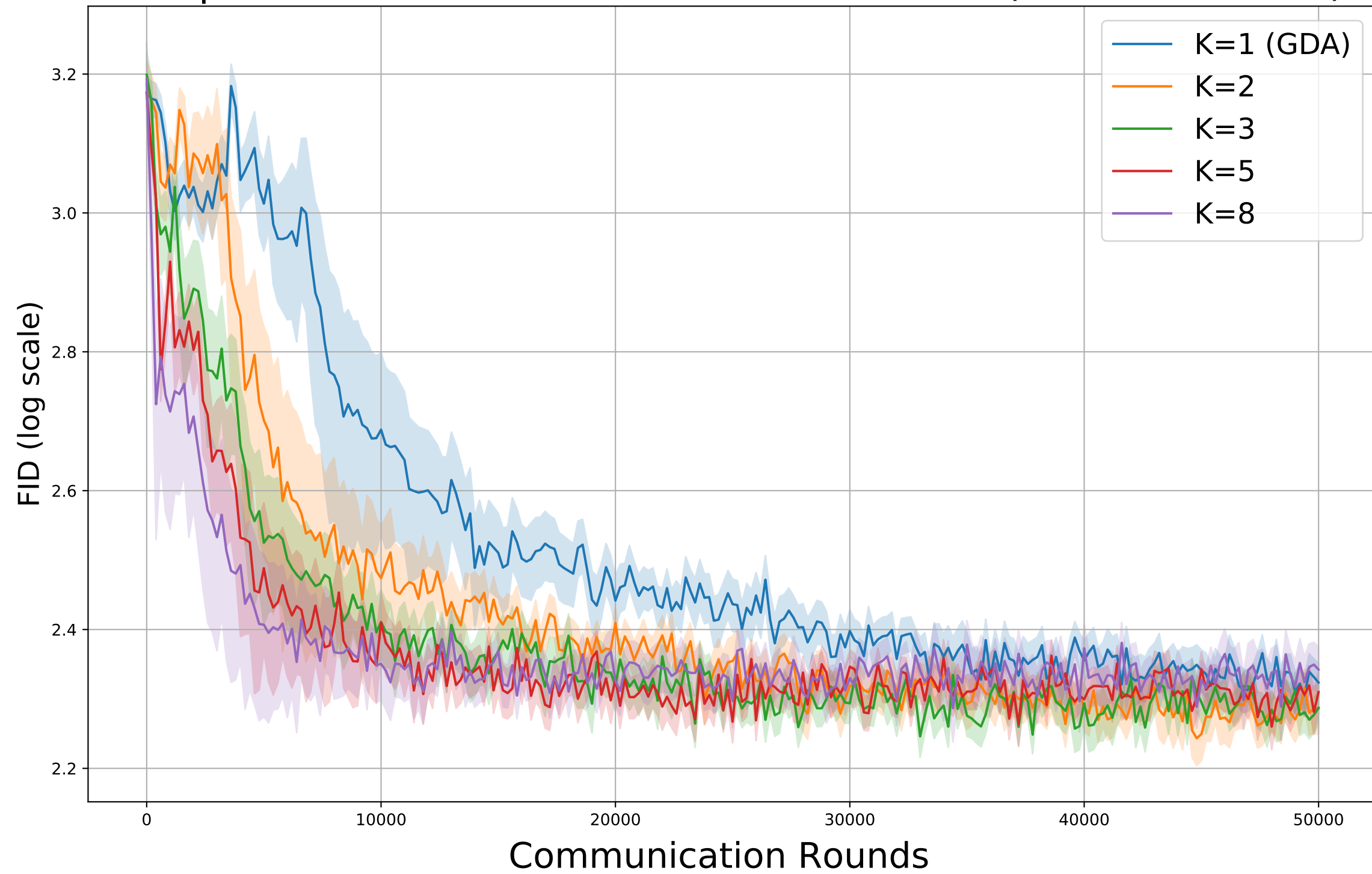
Comparison of FID vs Communication Rounds (Dataset: cifar10)
