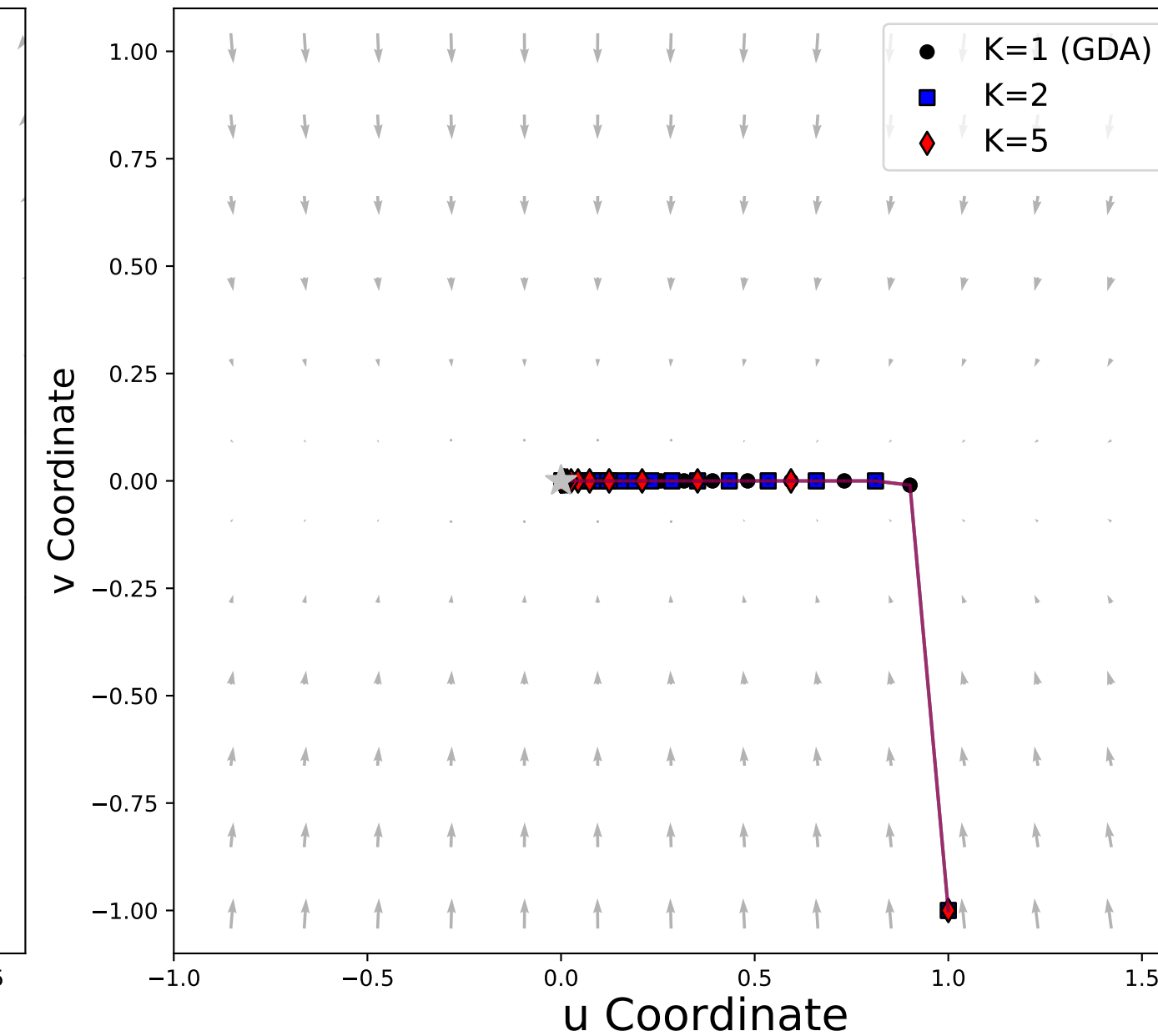
Trajectories for C=0
