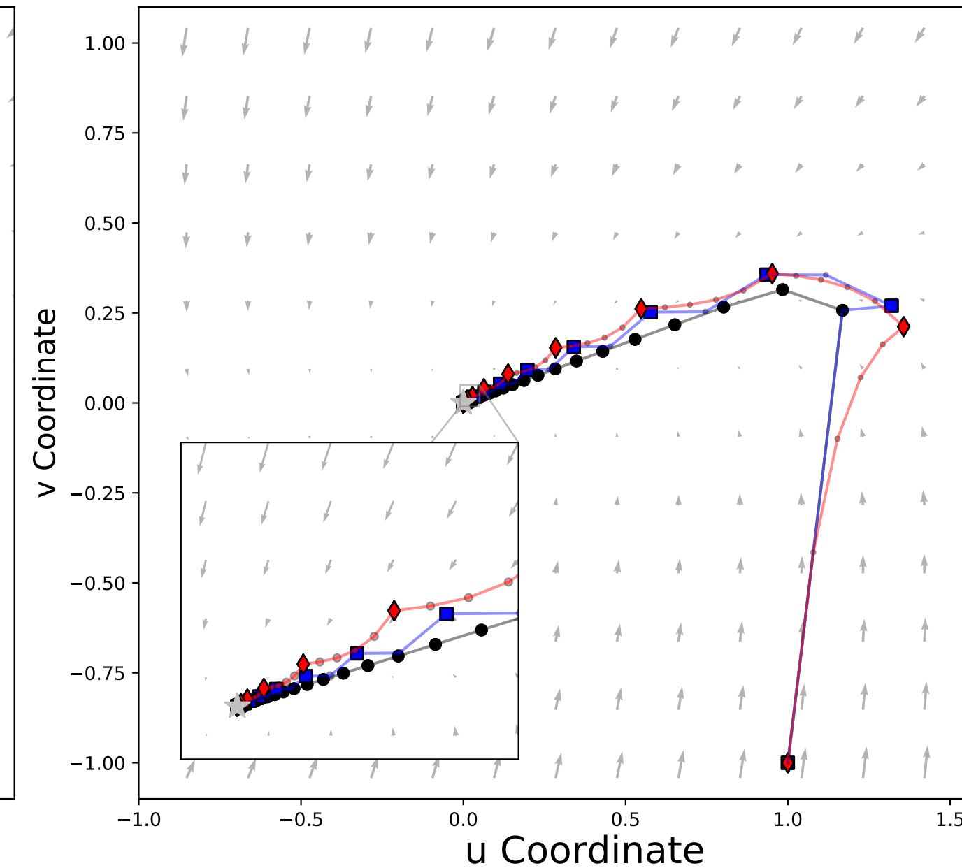
Trajectories for C=2.7
