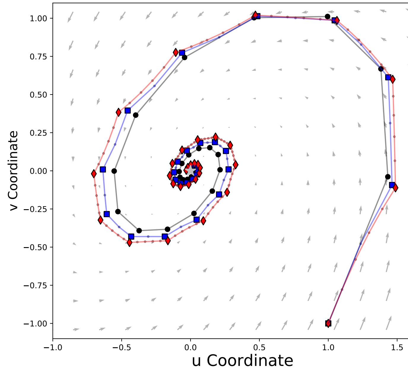
Trajectories for C=10
