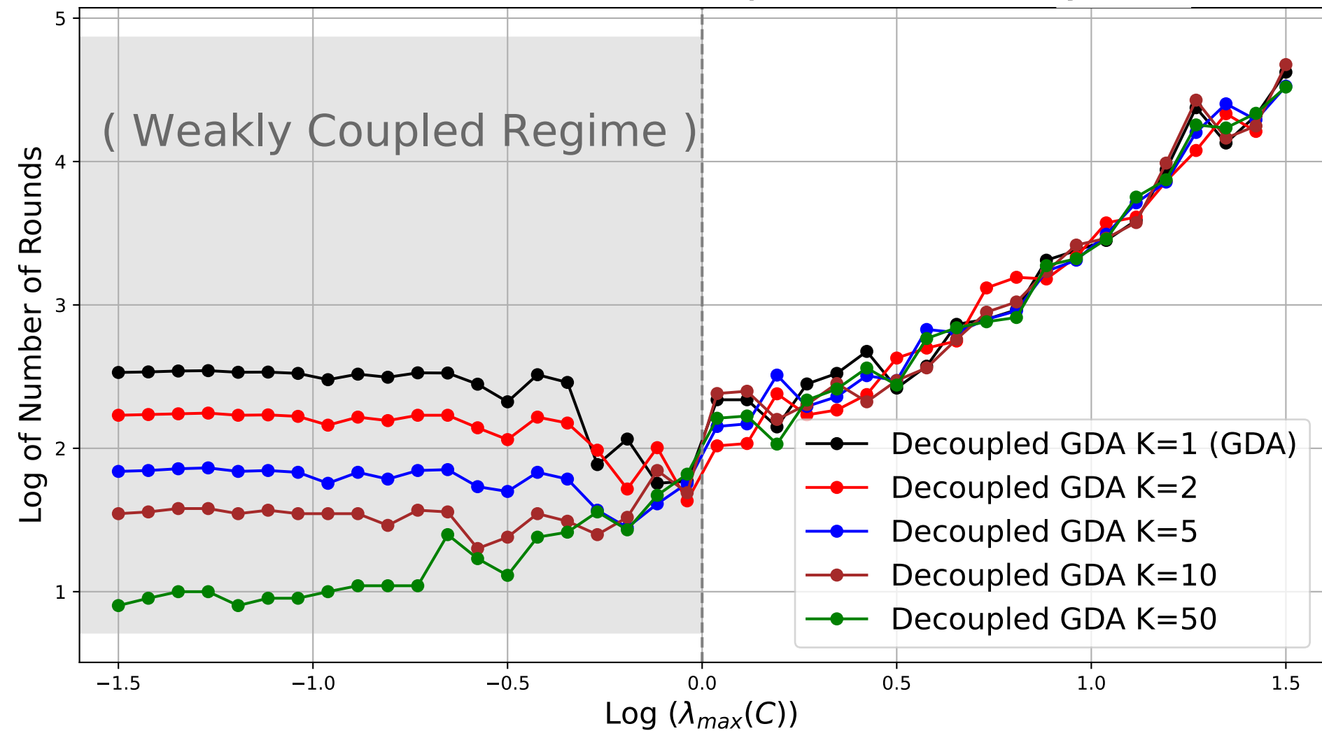
Number of Rounds to Reach Epsilon Accuracy vs \lambda_{max}(C)
