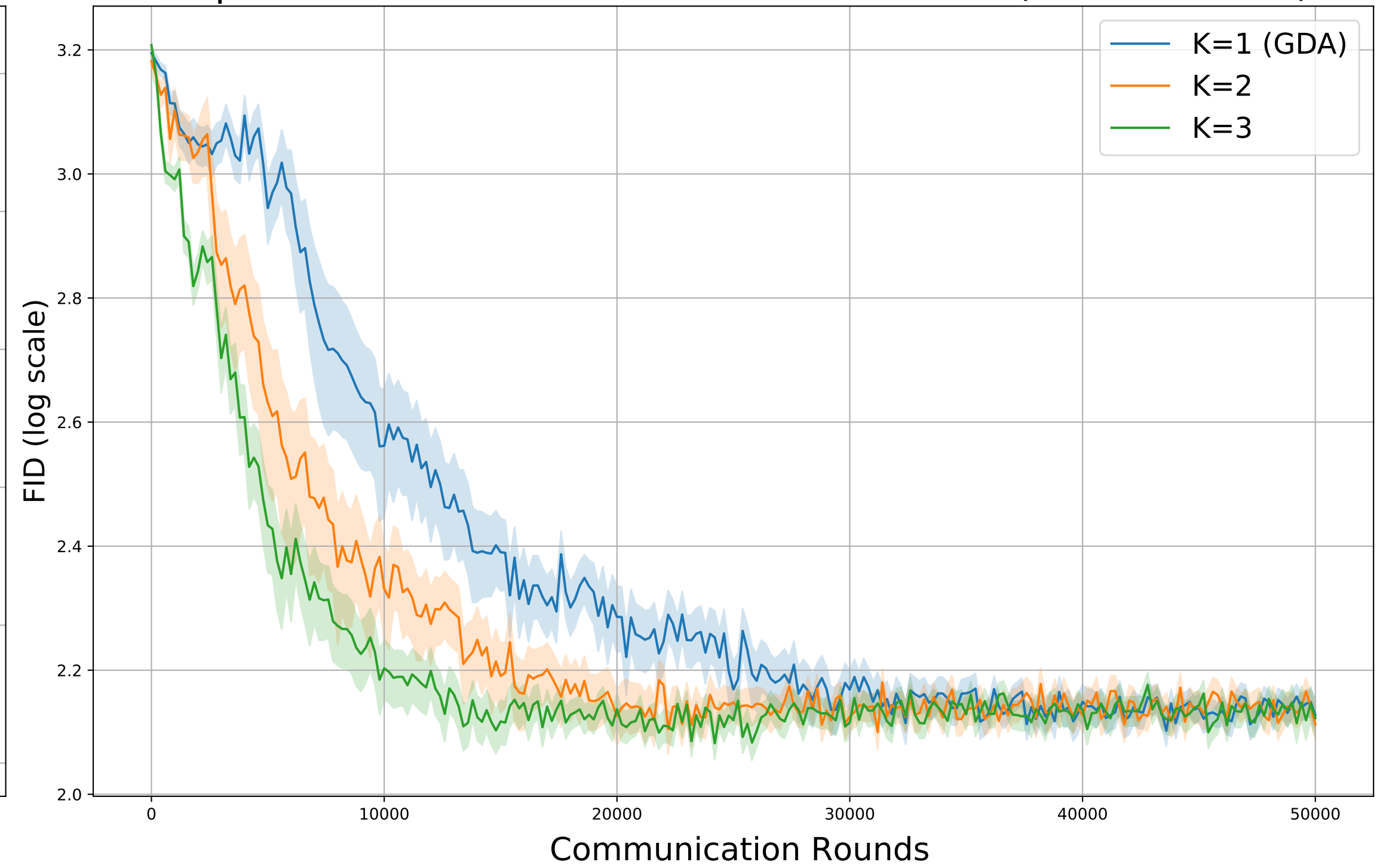
Comparison of FID vs Communication Rounds (Dataset: svhn)
