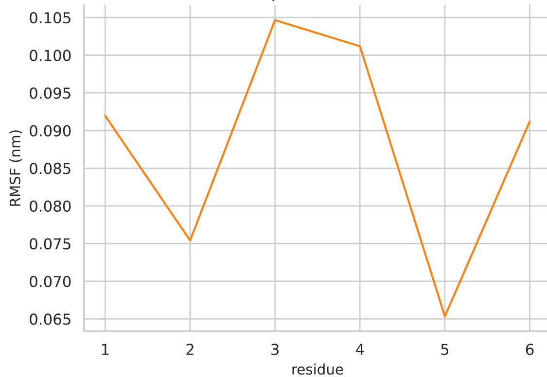
PHF6: per-residue RMSF
