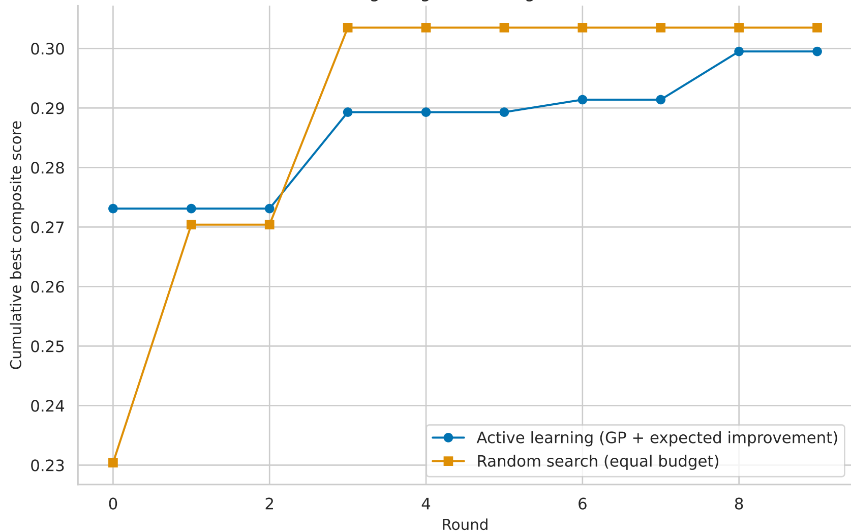
Design-engine learning curves
