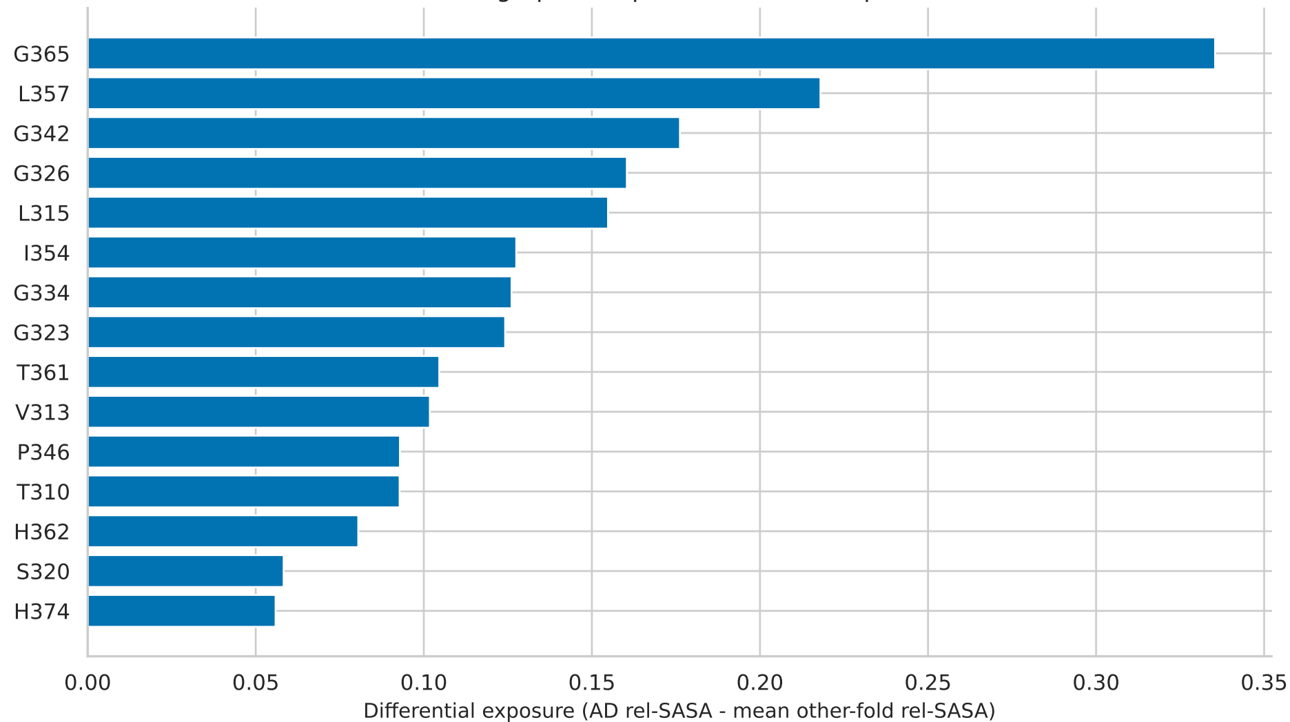
AD strain fingerprint: top AD-selective hotspot residues
