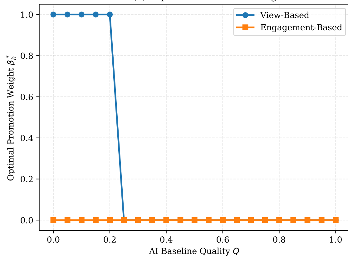
Panel (a): Optimal Promotion Weight
