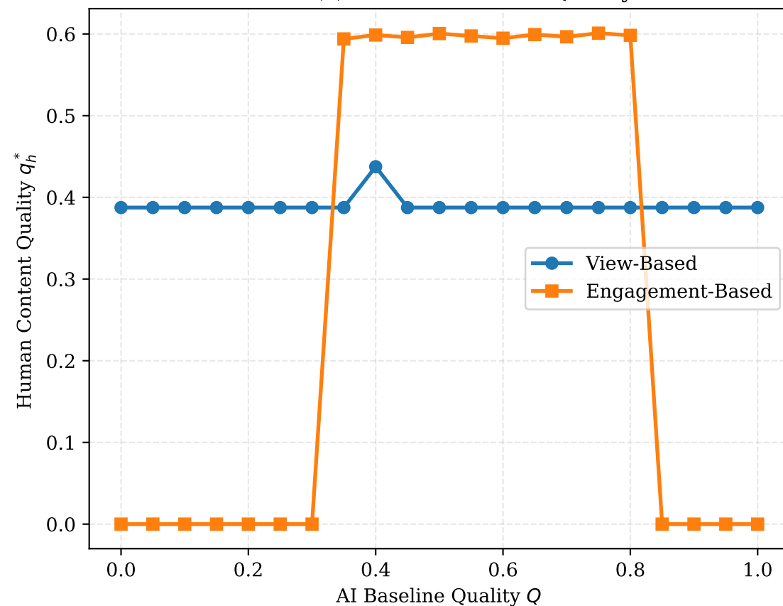
Panel (c): Human Content Quality
