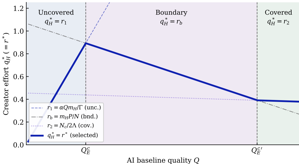
Engagement-based: equilibrium effort has three regions in Q (illustrative t = 2.4 , \alpha = 0.8 , \delta = 0.4 , \beta_H = 1/2 )
