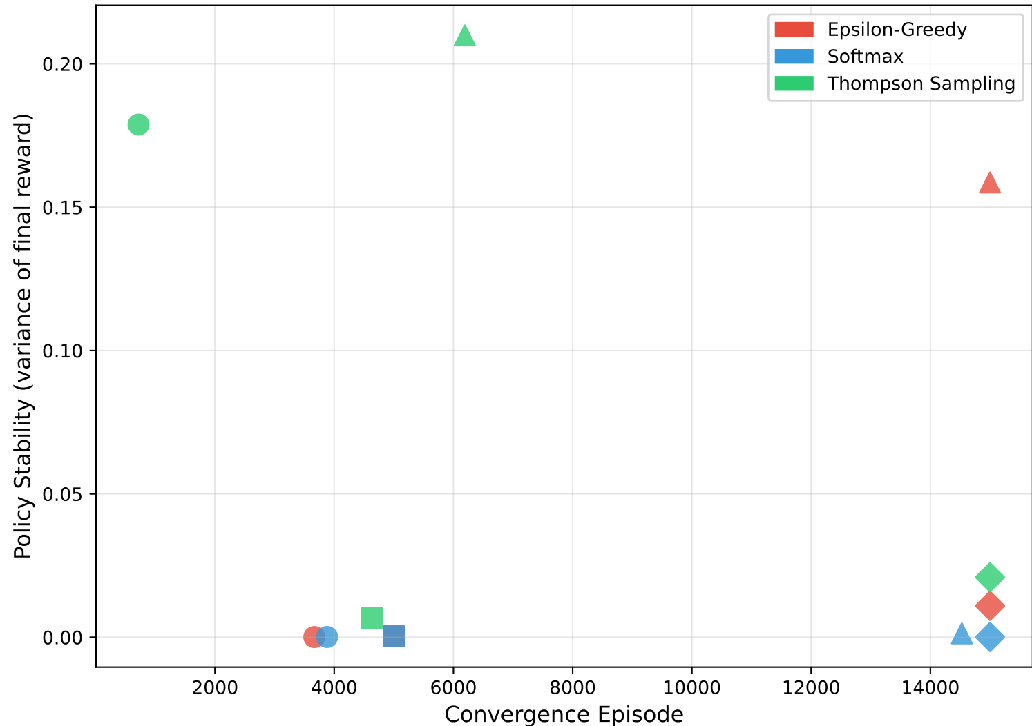
Convergence Speed vs. Policy Stability
