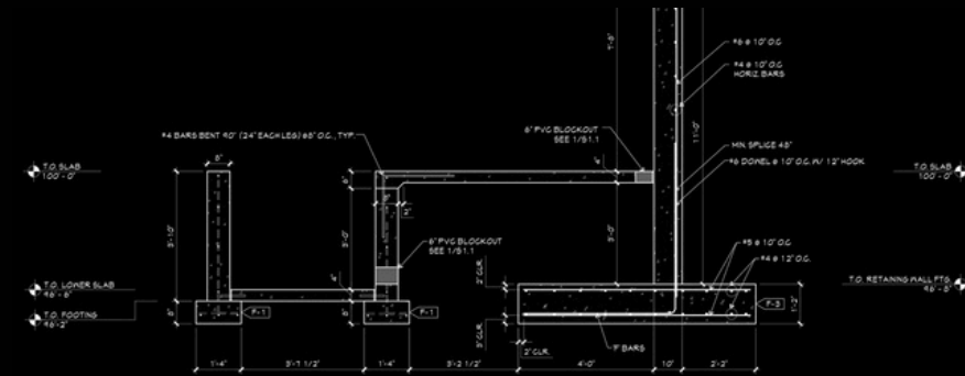
2 CONCRETE DETAIL SECTION 91.1 SCALE: 1/2" = 1'-0"
