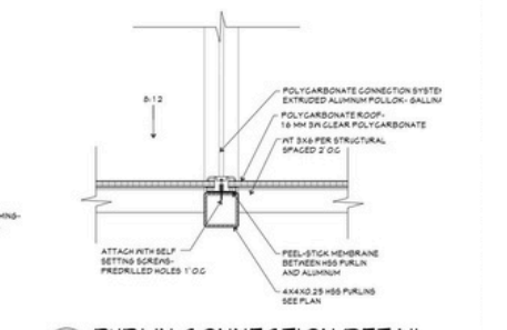
6 PURLIN CONNECTION DETAIL A3.1 SCALE: 1 1/2" = 1'-0"
