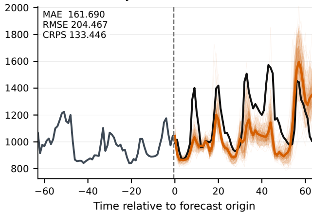
AirQuality — PETS-F (CG64 + Cal.)
