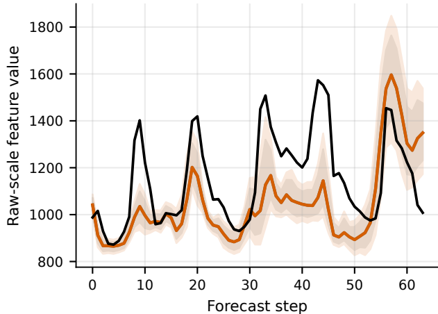
AirQuality — PETS spread calibration
