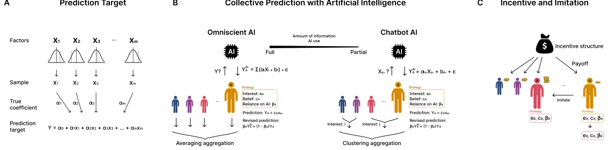
Figure 1: A schematic diagram of the model for individual and collective prediction in the presence of AI assistants. (A) The prediction target is modeled as a linear combination of causal factors, X_1, X_2, \dots, X_M : Y = \alpha_0 + \sum_{i=1}^M \alpha_i X_i . (B) Each player is characterized by three strategies: interest e_A , belief c_A , and reliance on AI \beta_A , where e_A \in \{0, \dots, M\} and X_0 = 1 . Players make predictions based on their interests and beliefs and subsequently revise them with AI assistance. We consider two types of AI, Chatbot AI and Omniscient AI, which differ in the amount of information available for generating predictions. Chatbot AI makes predictions based on user's interest: Y_A^{AI} = \alpha_{e_A} X_{e_A} + b_{e_A} + \epsilon_A . Omniscient AI makes predictions based on all causal factors: Y_A^{AI} = \sum_{i=0}^M (\alpha_i X_i + b_i) + \epsilon_A , where X_0 = 1 . For both cases, we assume \epsilon_A \sim \mathcal{N}(0, \tau) . (C) Players receive payoffs according to the incentive structure, and the population evolves through imitation of peers with higher payoffs.
