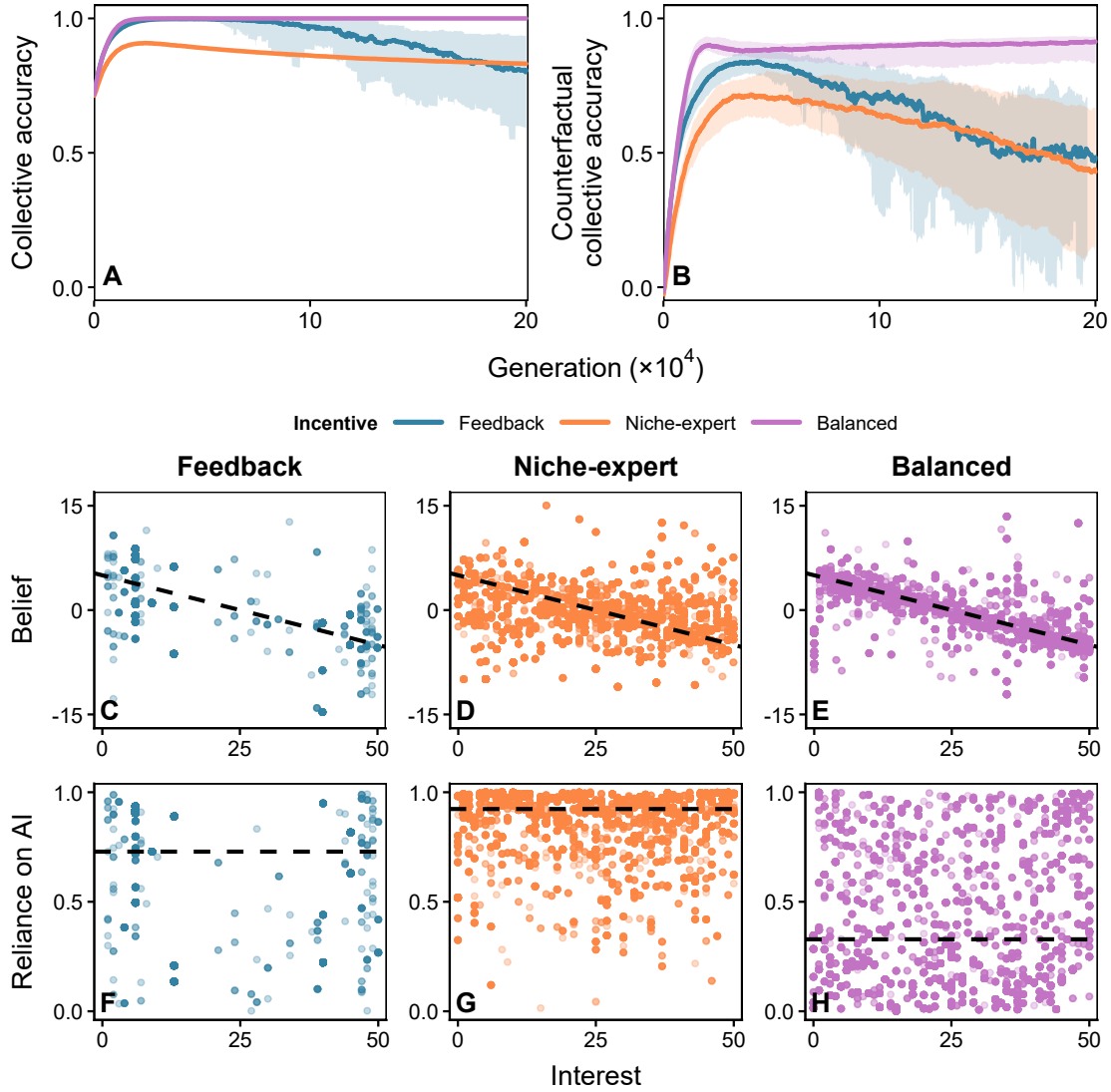
Figure 4: Balanced structure can promote collective intelligence. Trajectories of collective accuracy (A) and counterfactual collective accuracy (B) under three incentive structures (feedback, niche-expert, and balanced) with Chatbot AI. Each incentive structure was simulated for 30 independent replicates with randomly initialized player populations. Lines show the median across replicates, and shaded areas indicate the 95% simulation interval. Distributions of individual interest and belief (C-E) and of interest and reliance on AI (F-H) after 200,000 generations in one representative replicate. Each point represents an individual. Dashed lines in panels C-E represent the true coefficients ( \alpha_i ) of the prediction target. Dashed horizontal lines in panels F-H indicate the median reliance on AI. Prediction target parameters: M = 50 , \alpha_i = 5 - 0.2i , and \sigma_i \sim U(0, 3) . Evolutionary parameters: s = 50 and \mu = 0 . Population parameters: N = 10,000 , c_A \sim \mathcal{N}(0, 5^2) , and \beta_A \sim U(0, 1) . AI parameters: b_i = 0.4 and \tau = 0.3 .
