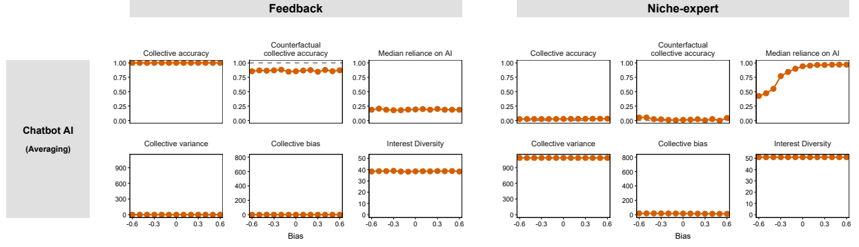
Figure S10: Chatbot AI with averaging aggregation has a limited influence on CI.
