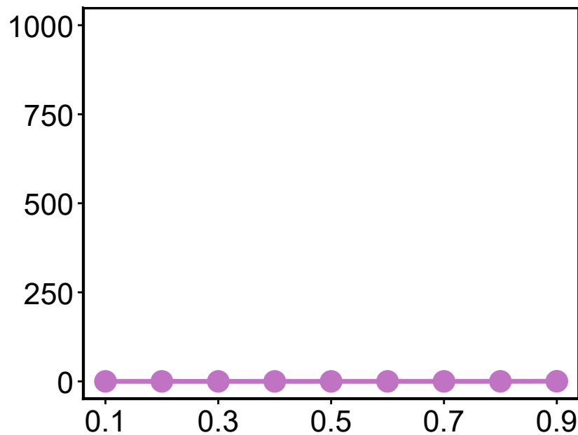
Collective variance
