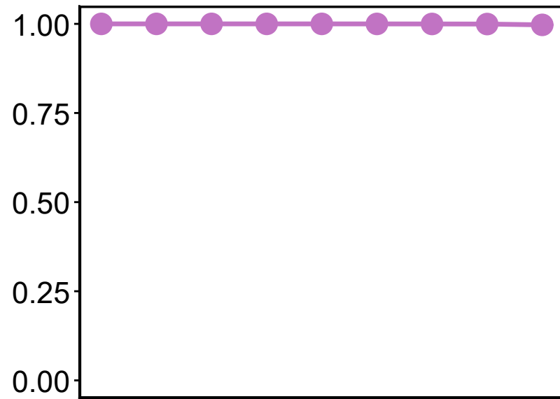
Collective accuracy
