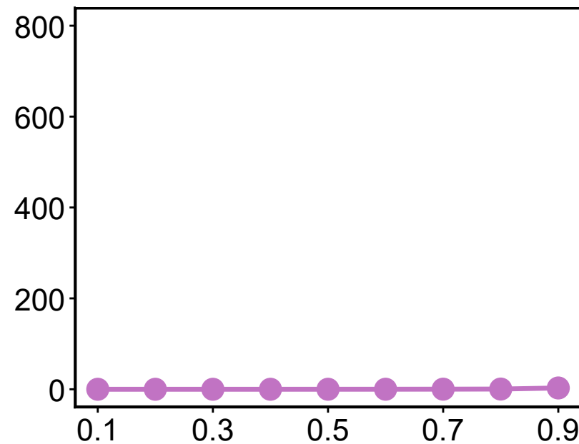
Collective bias
