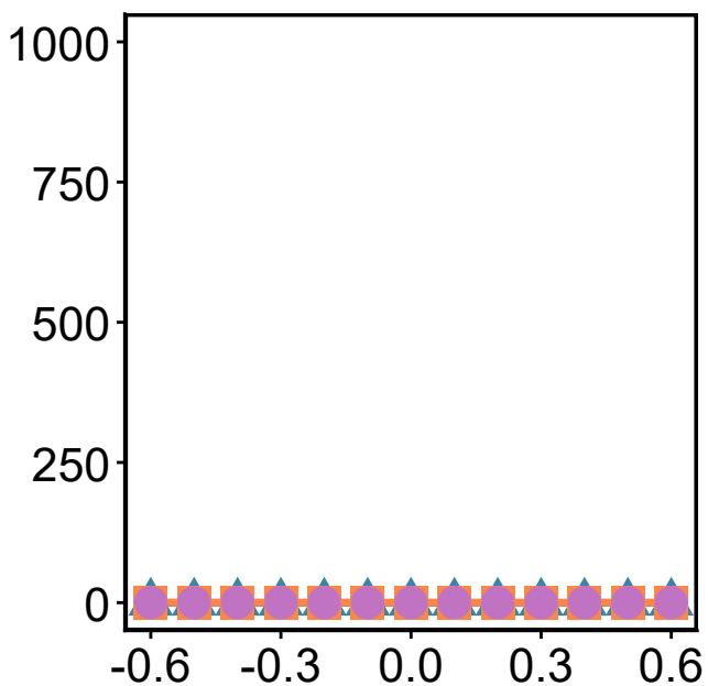
Collective variance
