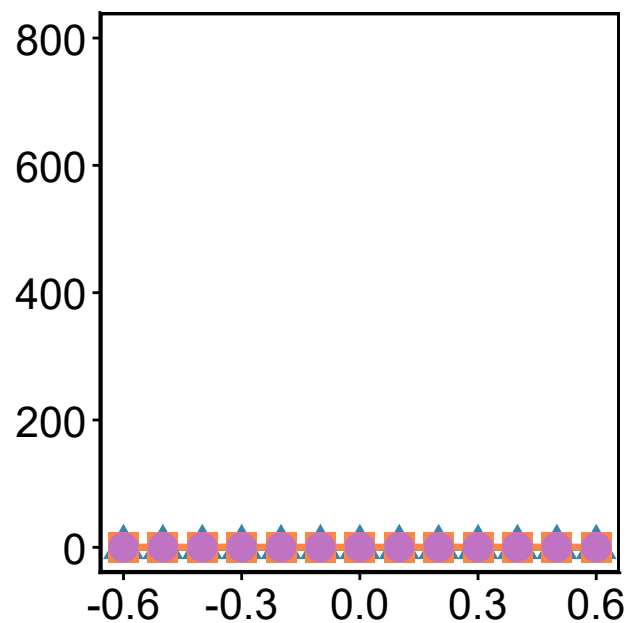
Collective bias
