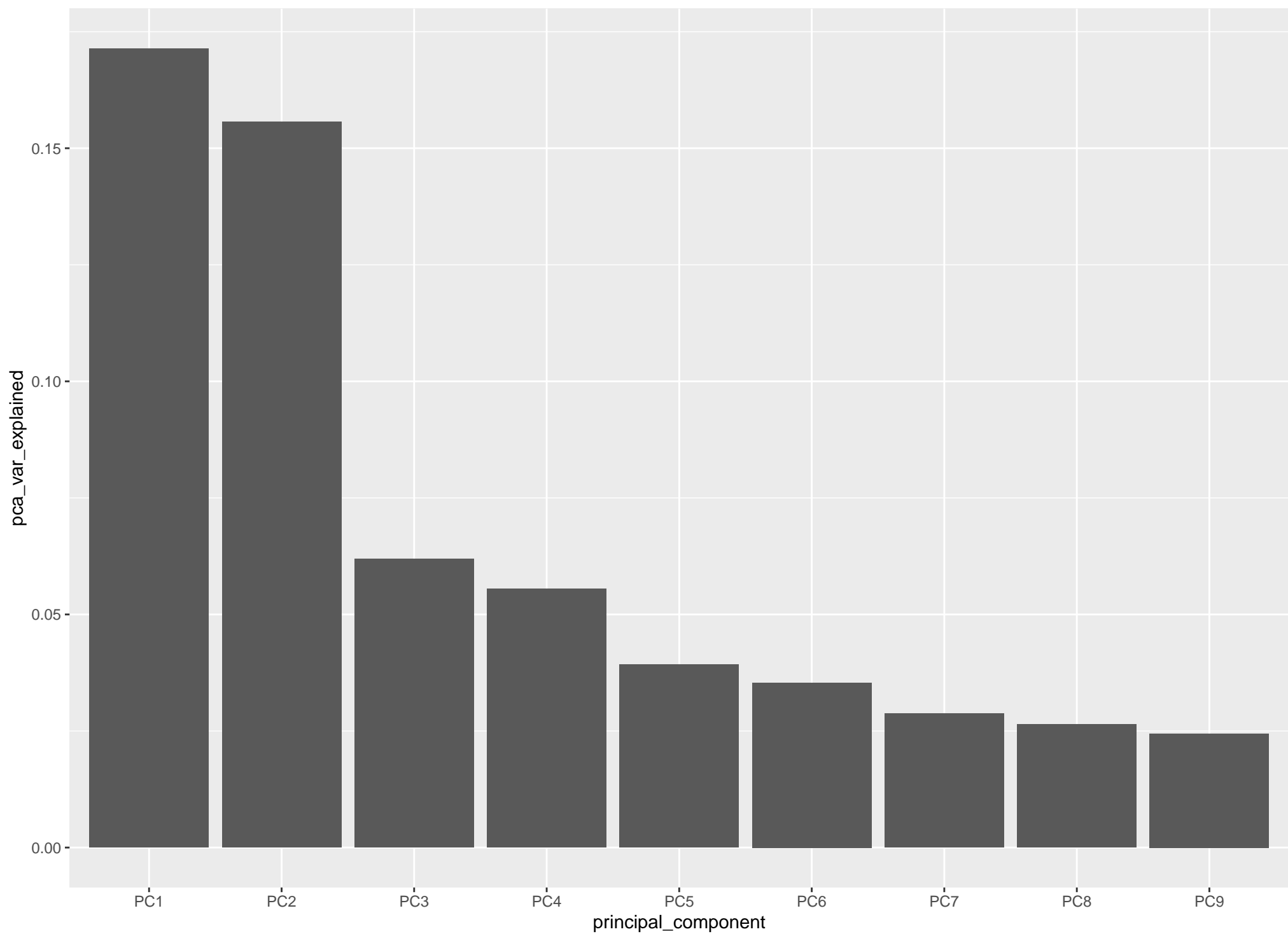
Scree Plot – % Variance Explained
