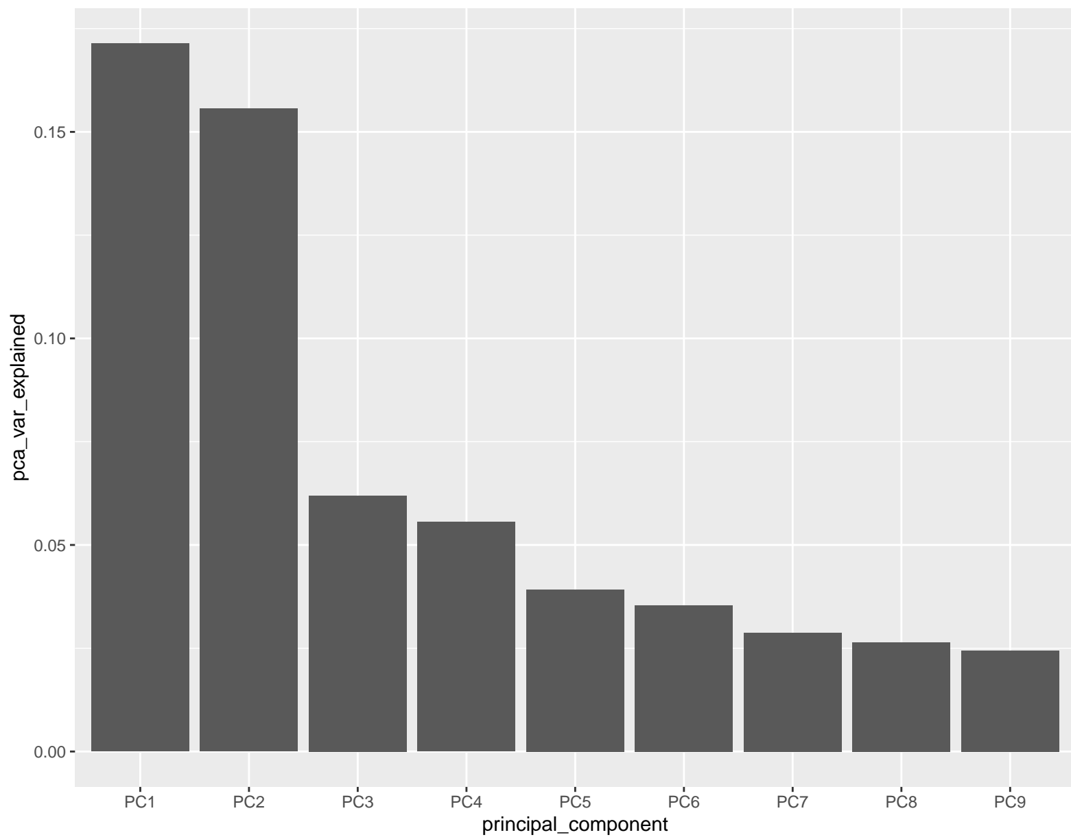
Scree Plot – % Variance Explained
