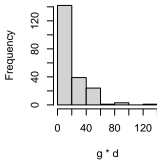
Histogram of g * d
