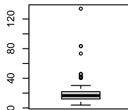
Boxplot of w=g*d
