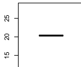
Boxplot of d
