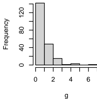
Histogram of g
