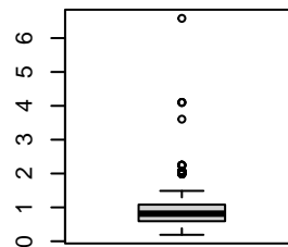
Boxplot of g
