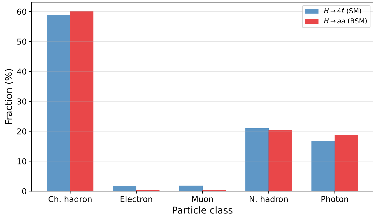
Particle Class Fractions: SM vs BSM
