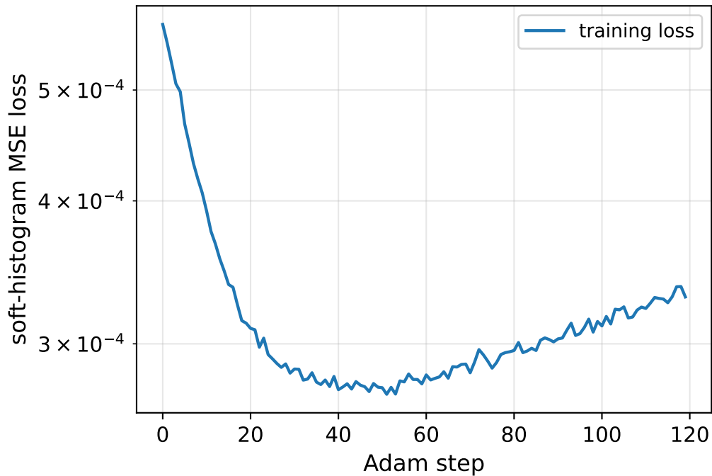
Loss trajectory
