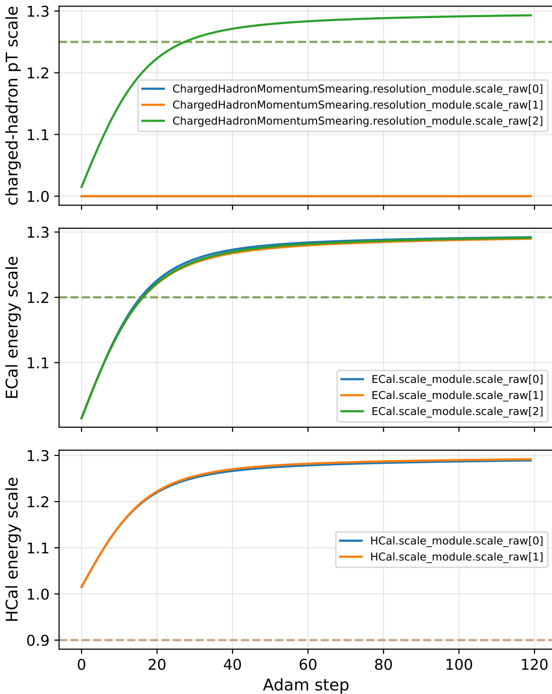
Scale-parameter drift during Adam fit
