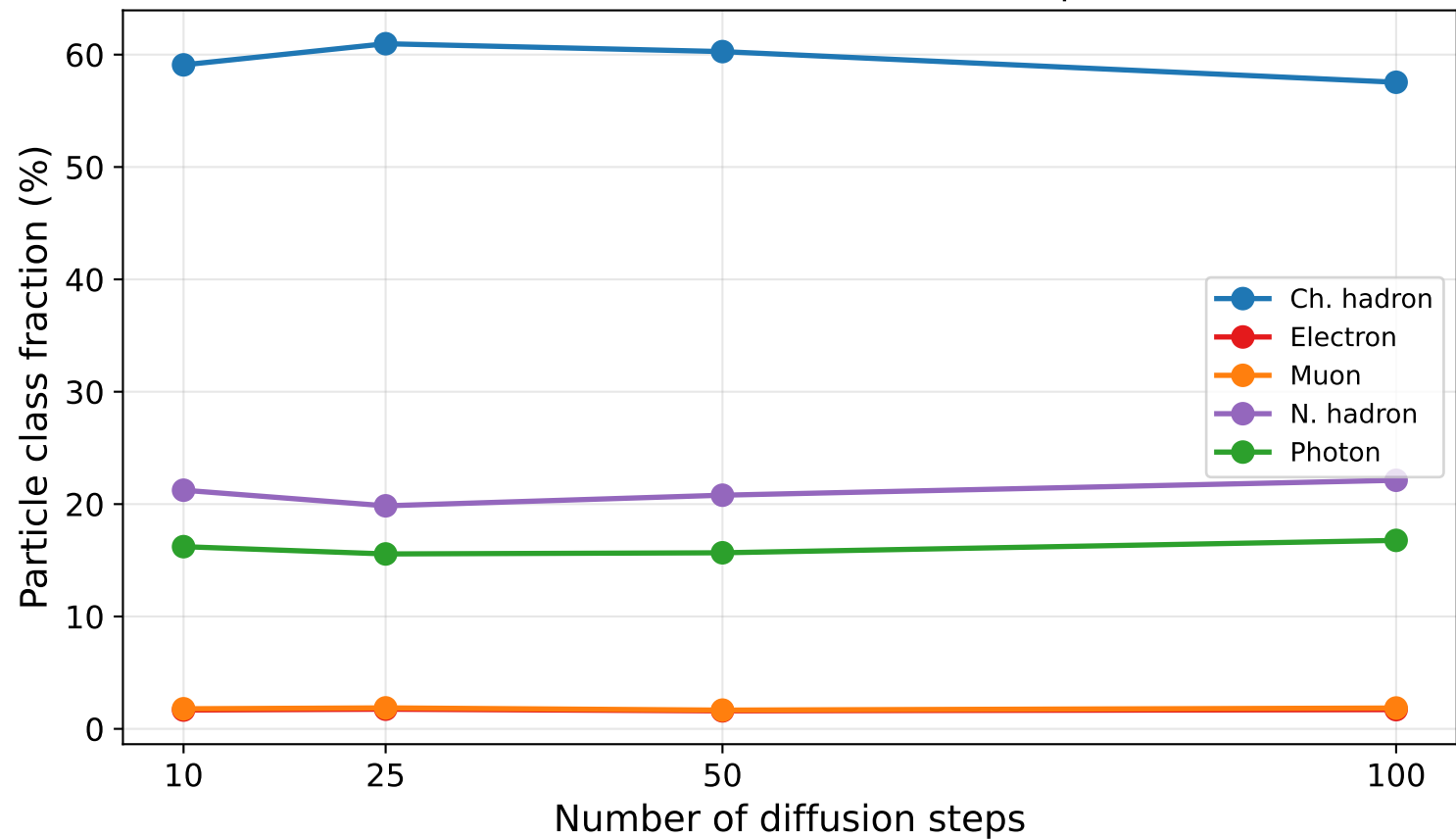
Particle Class Fractions vs. Diffusion Steps ( H \rightarrow 4\ell )
