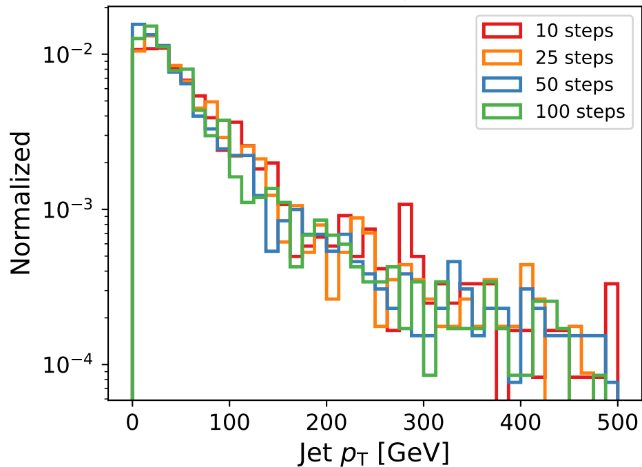
(a) Jet p_T
