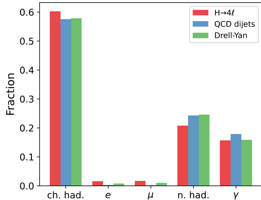
(c) Particle class fractions
