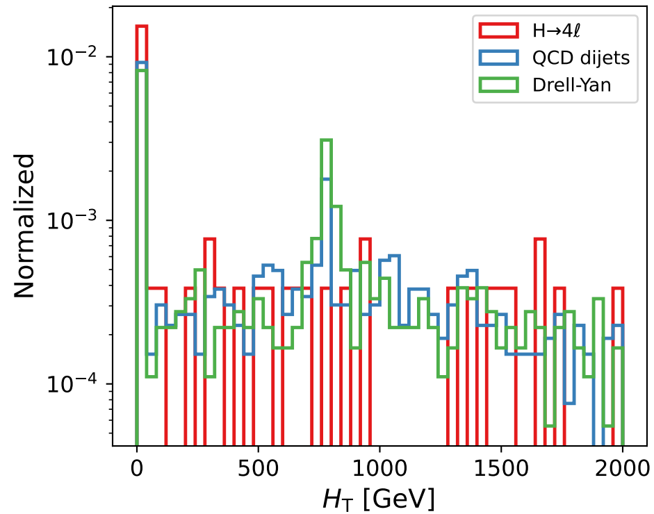
(a) H_T
