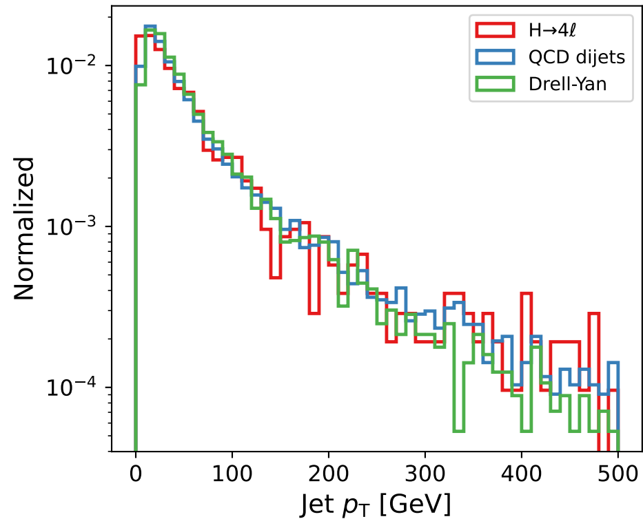
(a) Anti- k_t jet p_T
