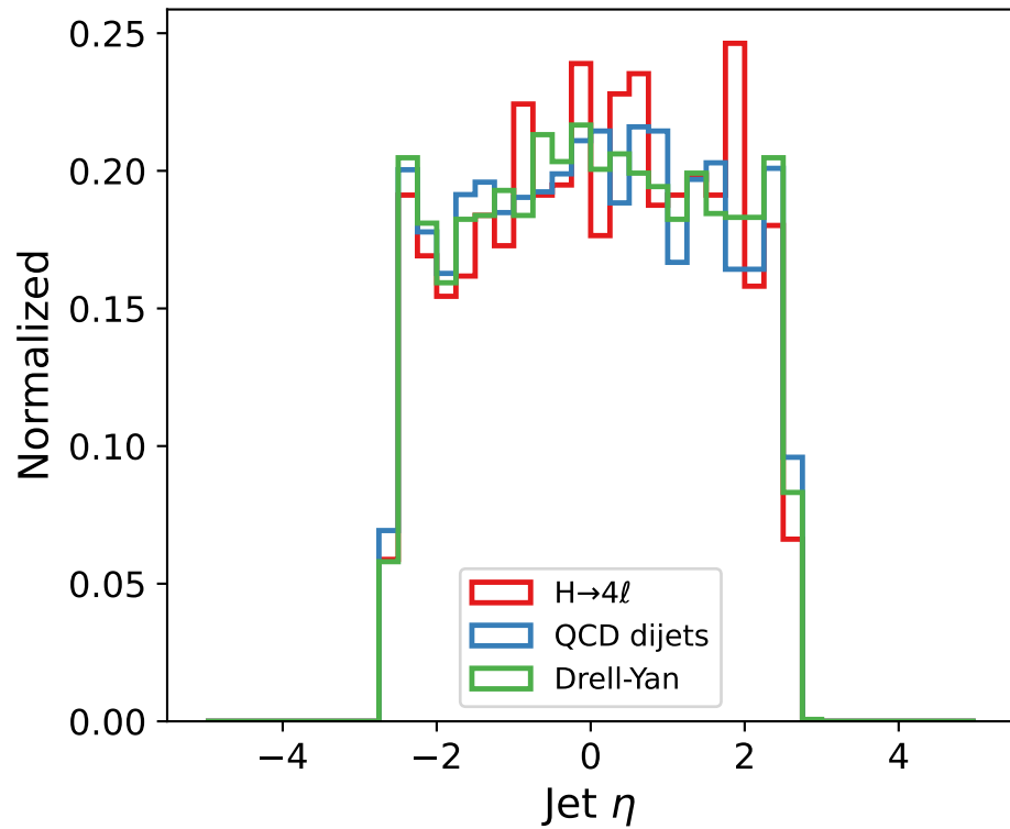
(b) Anti- k_t jet \eta
