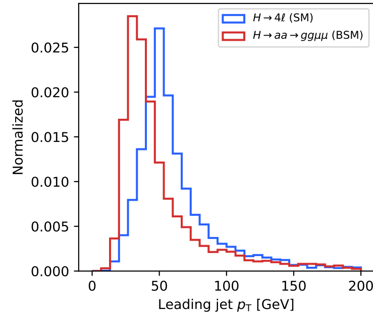
(c) Leading jet p_T
