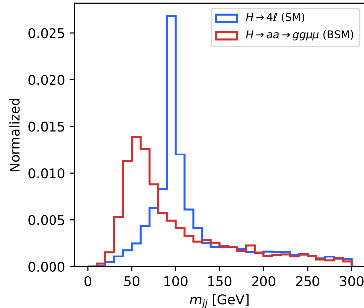
(a) Dijet invariant mass m_{jj}
