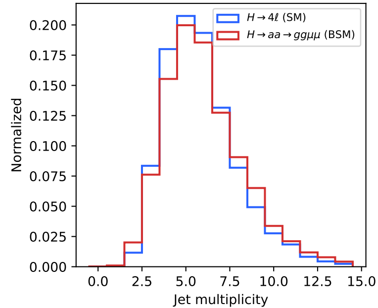
(b) Anti- k_t jet multiplicity
