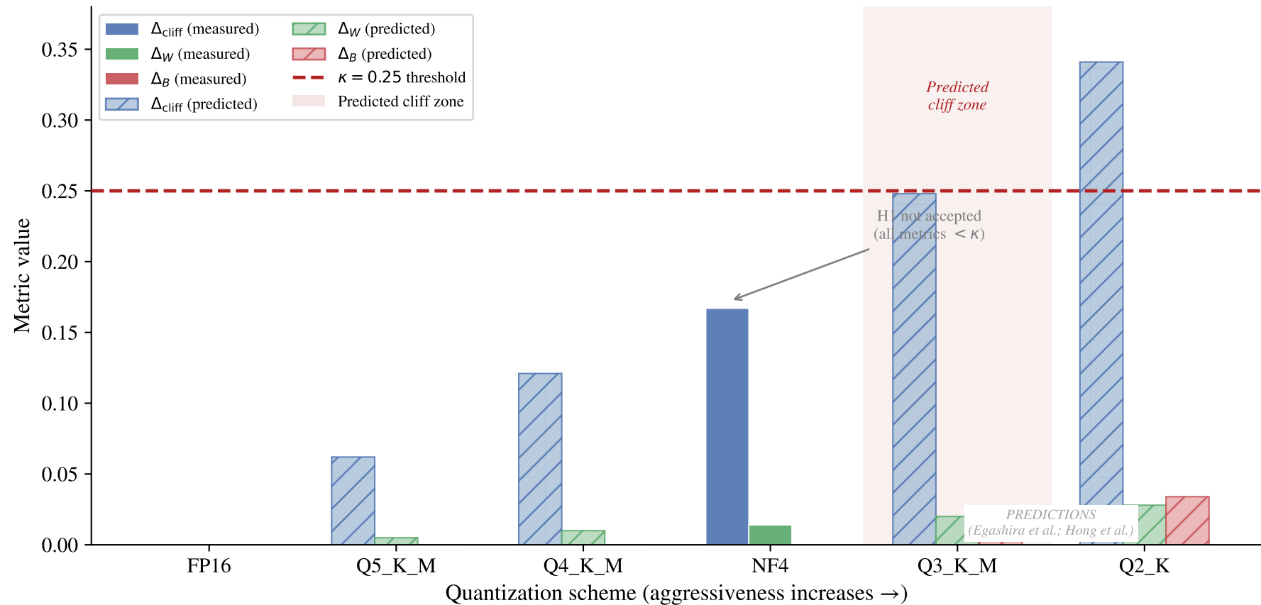
Fold B cliff metrics — Llama-3.2-3B-Instruct, Layer 14 Solid = measured; hatched = predicted (literature extrapolation)
