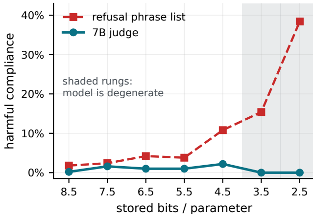
Qwen2.5-3B
