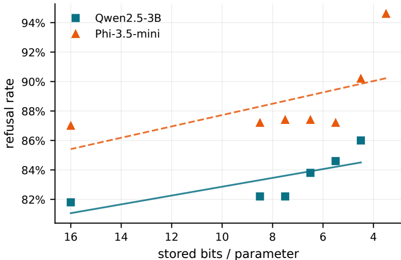
Refusal rises as precision falls, while output stays coherent
