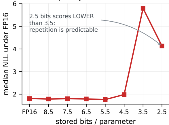
Perplexity is not monotone
