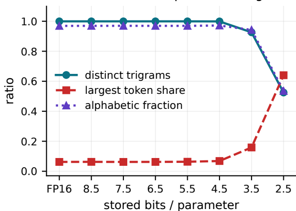
Surface statistics separate the regimes
