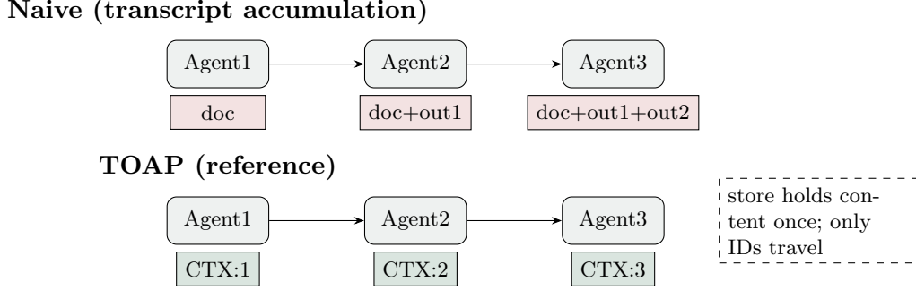
Figure 7: Token-flow contrast: naive prompts grow with depth; references stay flat.
