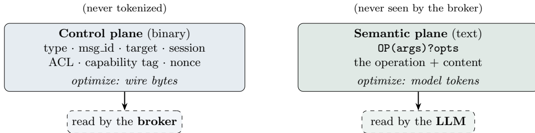
Figure 5: Two-plane message format. Each plane is encoded for its single reader and cost function: the broker reads the byte-optimized control plane and never tokenizes the payload; the LLM reads the tokenizer-aligned semantic plane and never sees the control header.
