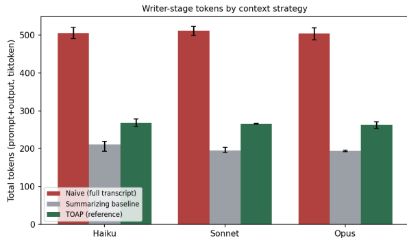
Figure 8: Writer tokens by strategy (error = min-max). Summary < TOAP < naive.
