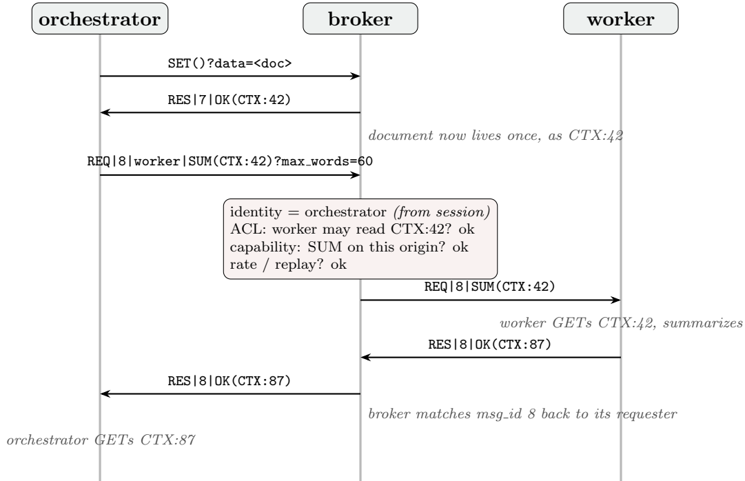
Figure 2: One request, traced through the stack. The document is stored once and thereafter referenced by id; the inter-agent message carries CTX:42 , not the document. The broker stamps the sender’s identity from its session, runs the four security checks, and routes by target. The worker replies to msg_id 8 , and the broker uses that id to return the reply to whoever sent request 8 — so the worker never names, and could never forge, the requester.
