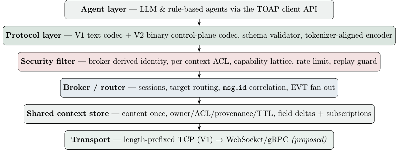
Figure 4: TOAP layered architecture. Identity/trust are broker-owned, never claimed on the wire.
