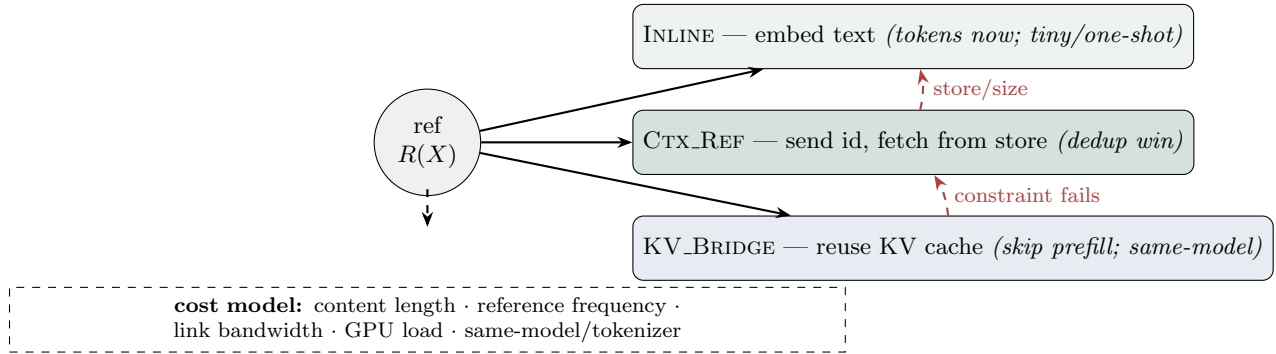
Figure 6: Reference materialization spectrum: one logical reference, three materializations chosen per call by a cost model, with graceful degradation \text{KV\_BRIDGE} \rightarrow \text{CTX\_REF} \rightarrow \text{INLINE} when constraints fail. The same decision spans the token plane (resend vs. id) and the tensor plane (re-prefill vs. load KV).
