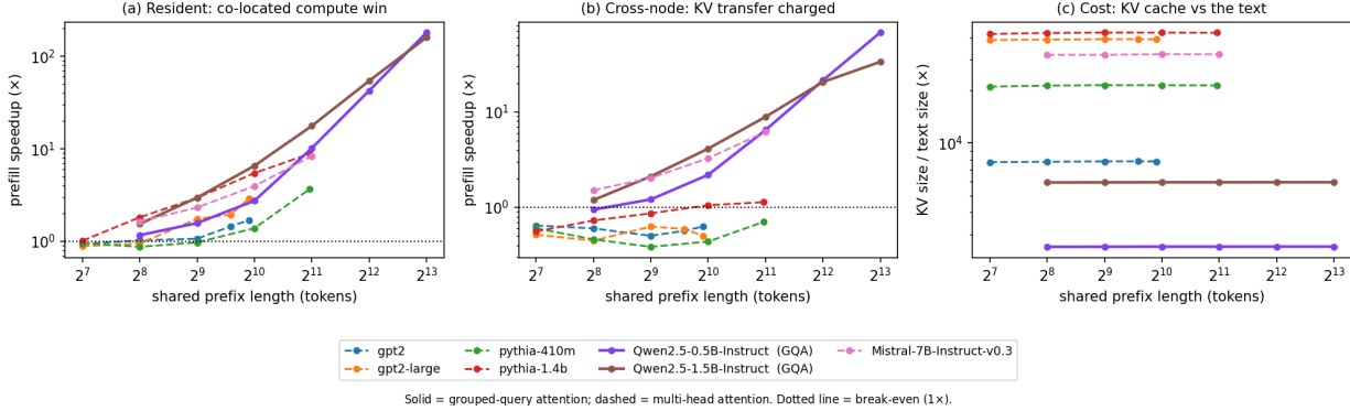
Figure 10: KV-bridge prefill reuse across seven models on an NVIDIA T4 (36 cells, log scales). (a) Resident speedup grows with prefix length and is dramatic for GQA models (solid), reaching \sim 180\times at 8k tokens. (b) With KV transfer charged, GQA stays above break-even while MHA (dashed) mostly does not. (c) The KV cache is thousands of times larger than the text, and far larger for MHA than GQA — the reason transfer cost flips the verdict by architecture.
