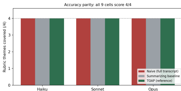
Figure 9: Accuracy parity: all nine cells 4/4 (the n=1 regression did not reproduce).
