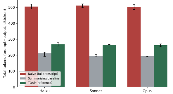
Writer-stage tokens by context strategy ( n=5 Haiku, n=3 Sonnet/Opus; error=min-max).
