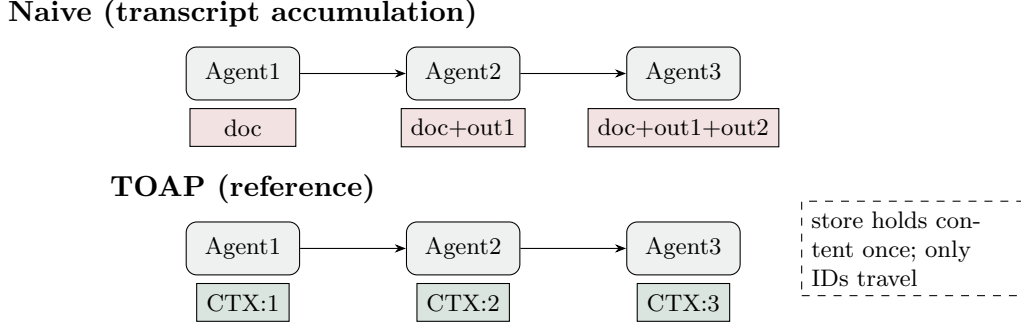
Figure 3: Token-flow contrast: naive prompts grow with depth; references stay flat.
