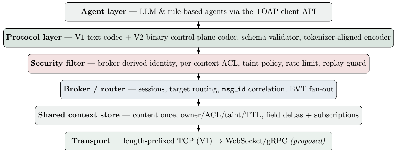
Figure 2: TOAP layered architecture. Identity/trust are broker-owned, never claimed on the wire.
