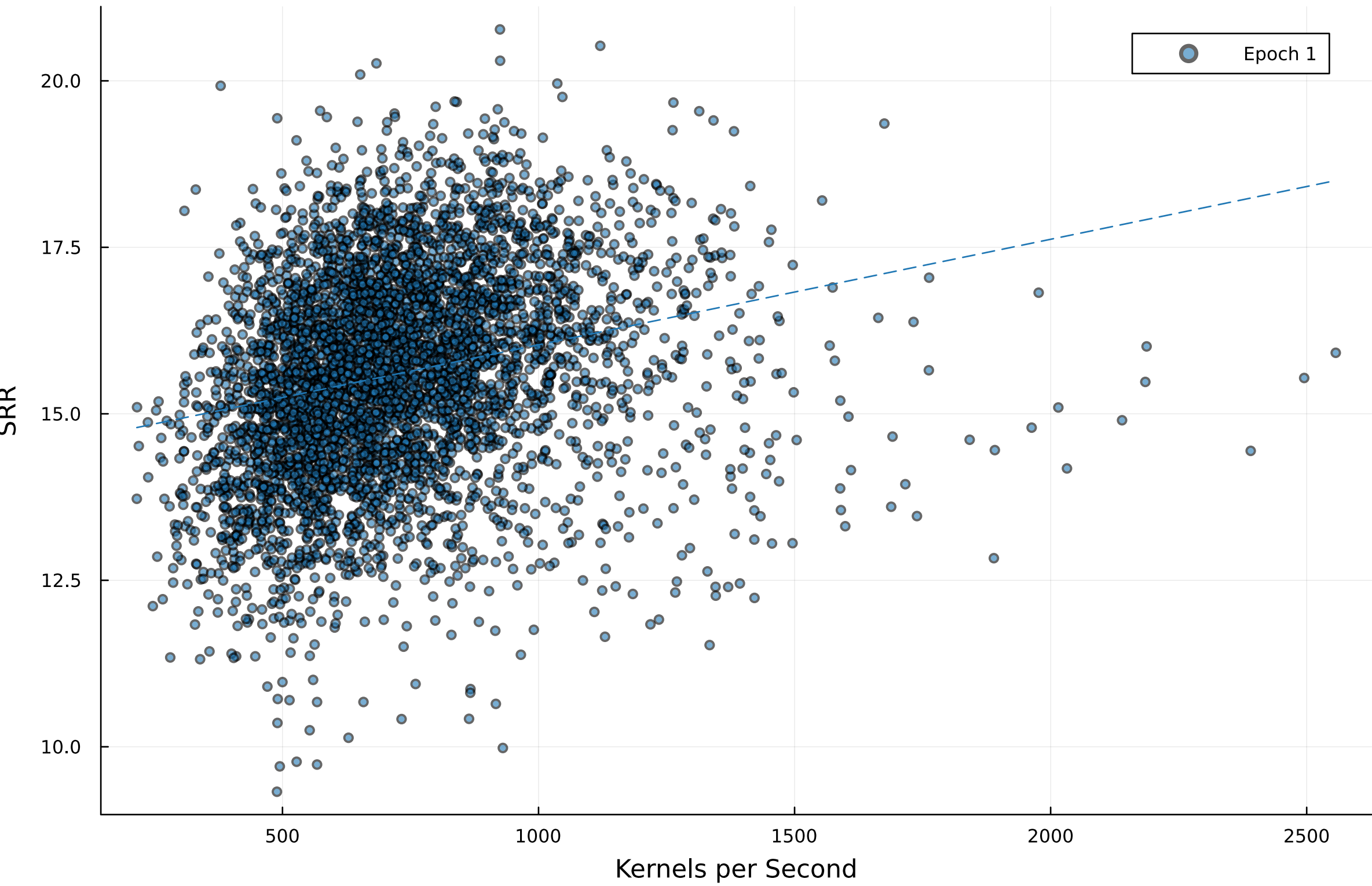
SRR vs Kernels/sec by Epoch
