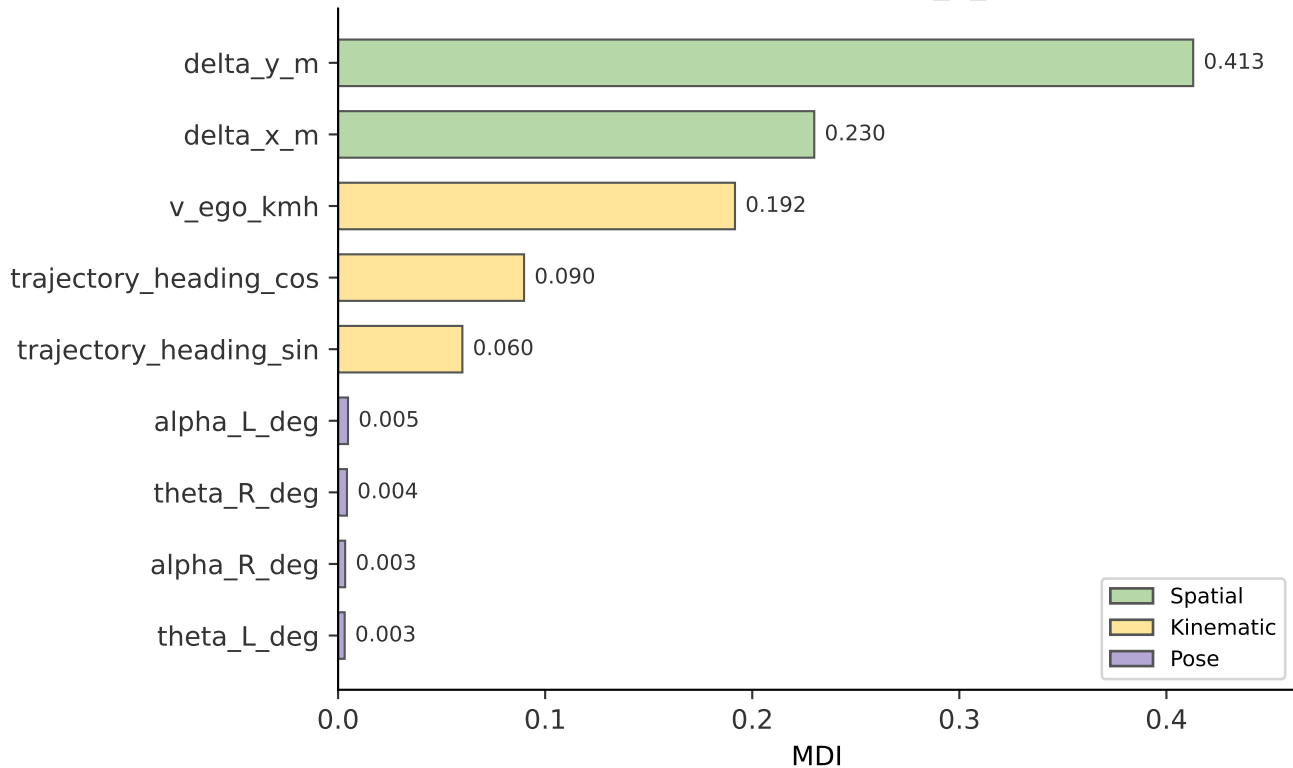
Feature importance — pie_9_heading
