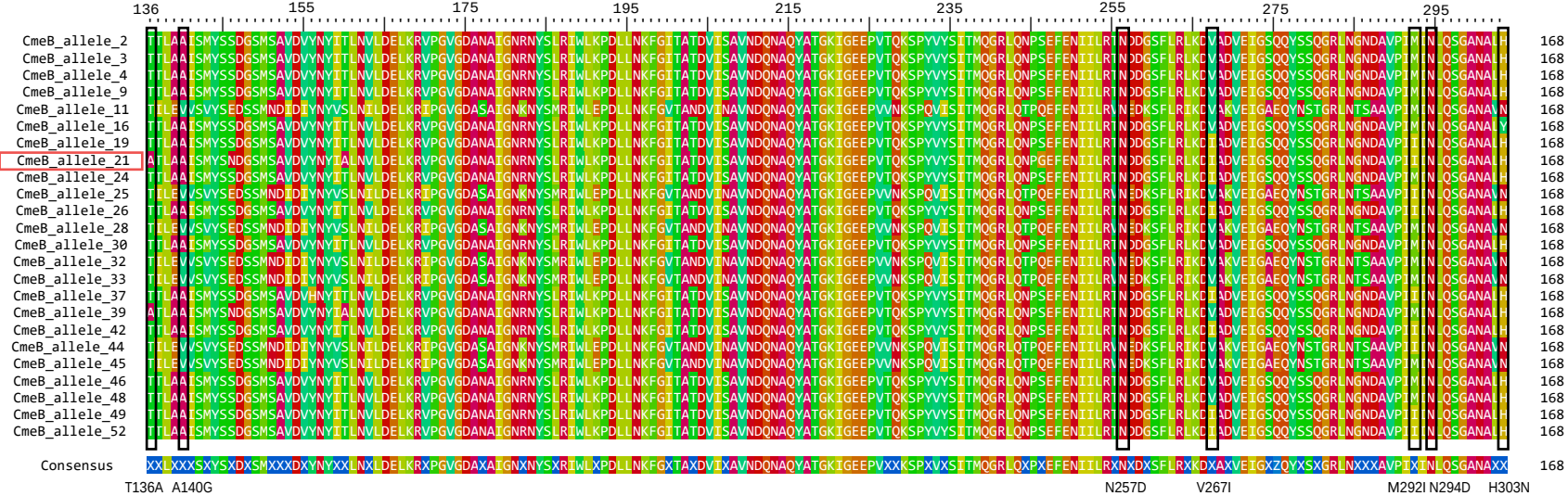
CmeB alignment C. jejuni — positions 136 to 303 (RE-CmeB mutation sites)
