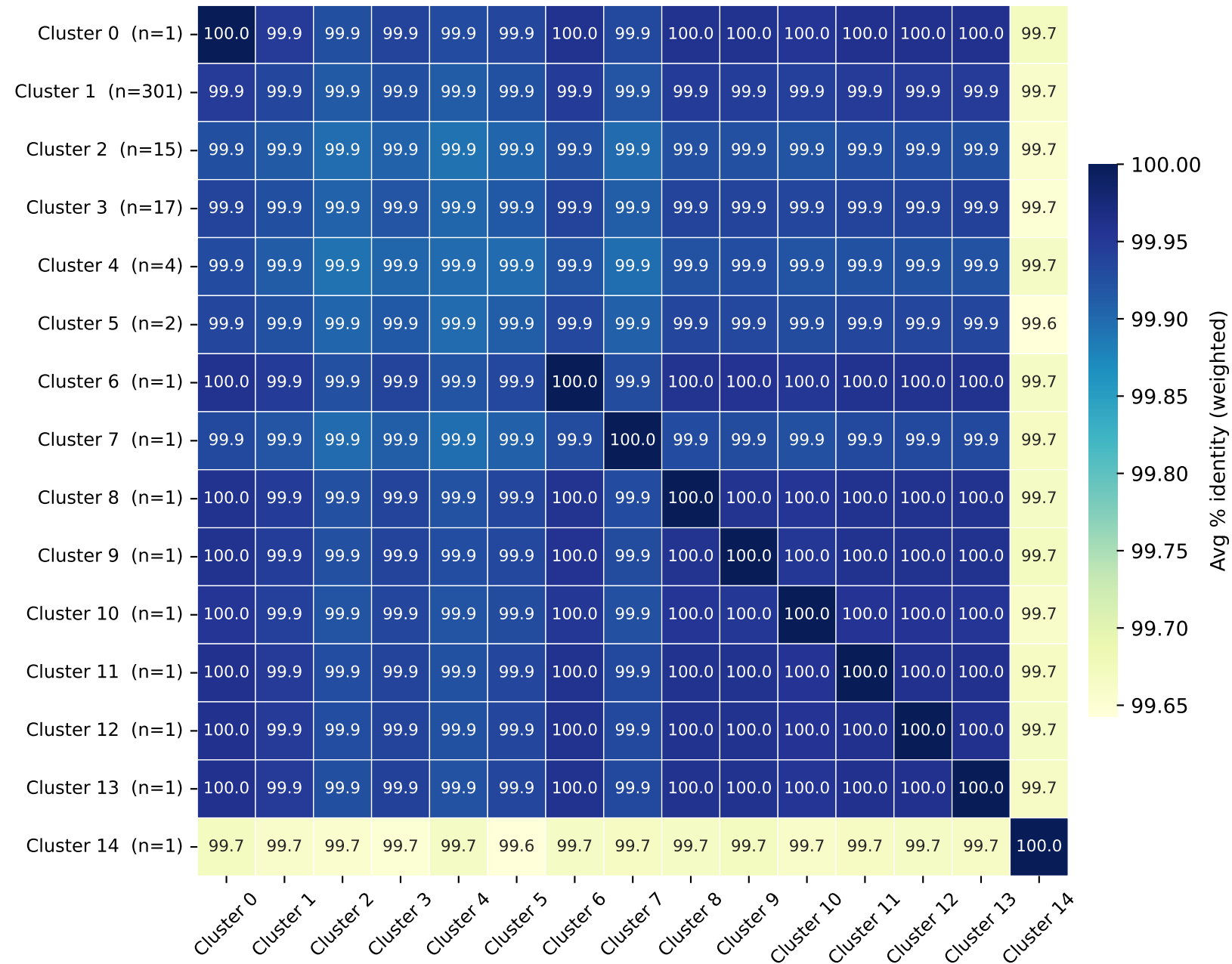
Average pairwise BLASTn identity between pVir plasmid clusters
