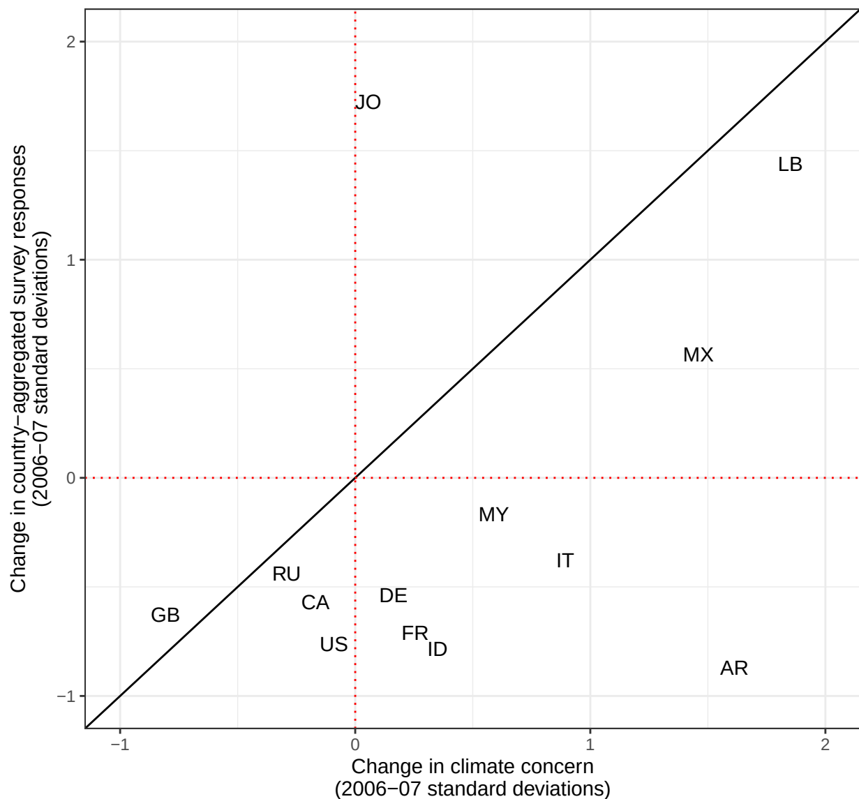
Change in worry_climatethreat_pew and climate concern estimates, 2006-07 --2014-15
