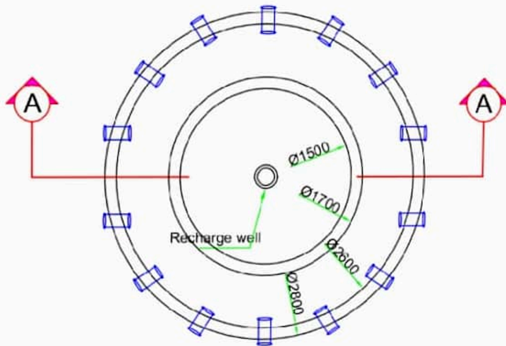
Plan of Rainwater recharge shaft
