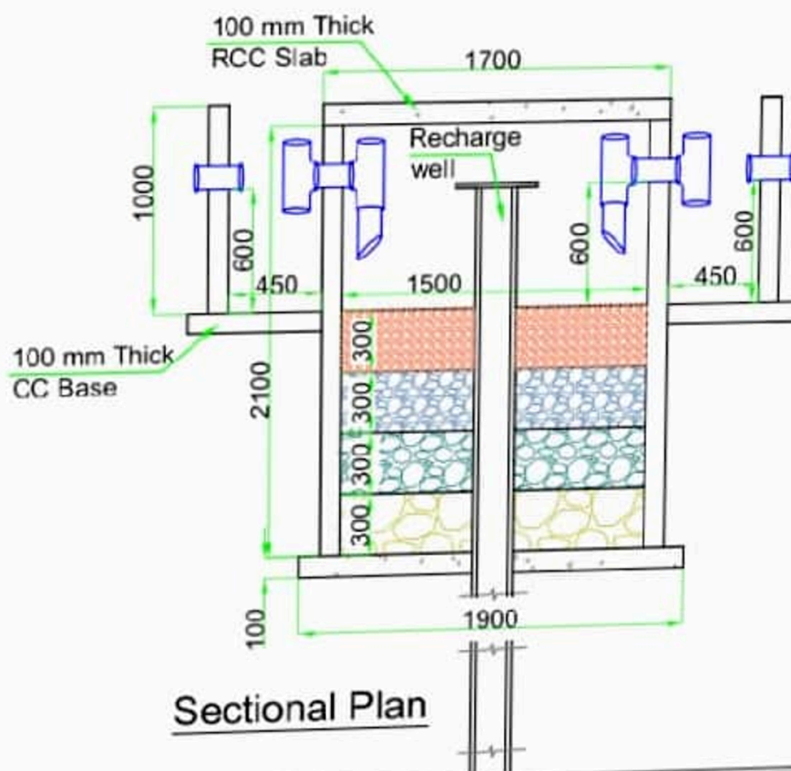
Plan of Rainwater recharge shaft
