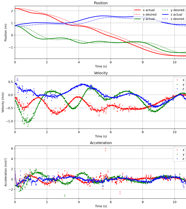
Fig. 2: Experimental tracking results for Maze 3.
