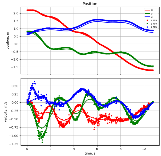
(c) Maze 3 Performance
