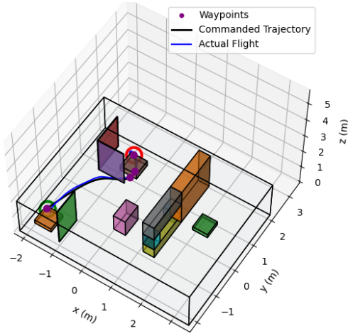
(a) Maze 1 Trajectory
