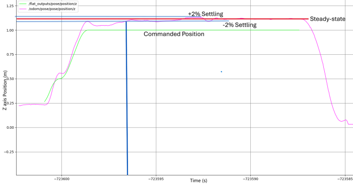
Fig. 1: Z-axis position response over time. The green curve represents the commanded position, while the purple curve represents the actual measured position. The \pm 2\% bounds are defined around the steady-state value of the actual response and are used to determine the settling time.
