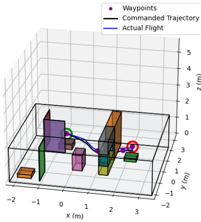
(b) Maze 2 Trajectory
