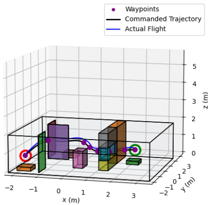
(c) Maze 3 Trajectory
