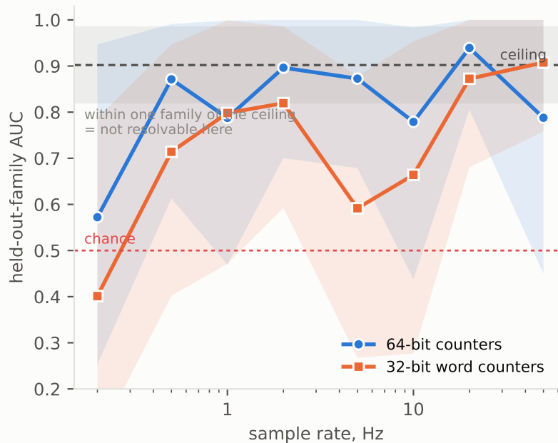
Detection vs how often we look
