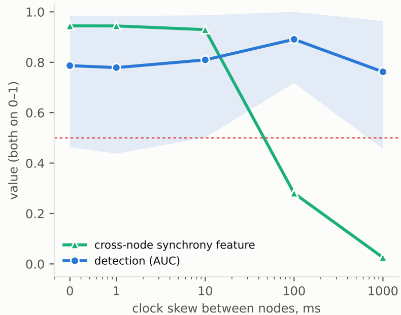
Clock skew kills the feature, not the detector
