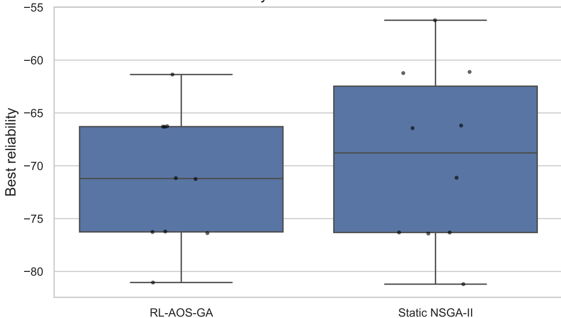
Best Reliability Distribution Across Seeds
