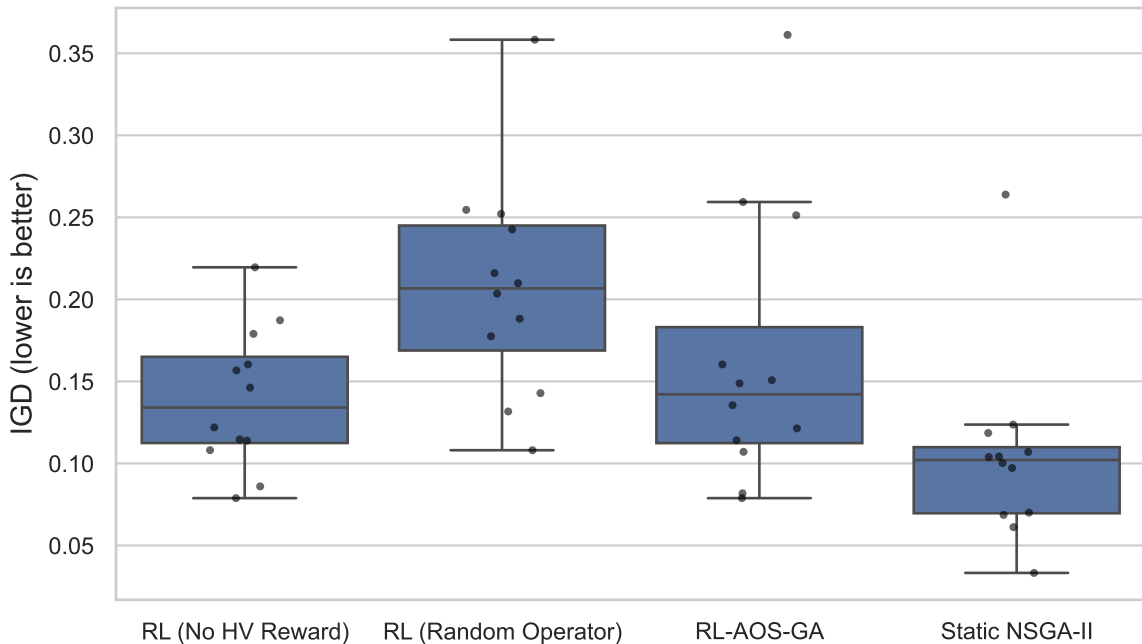
IGD Distribution Across Seeds
