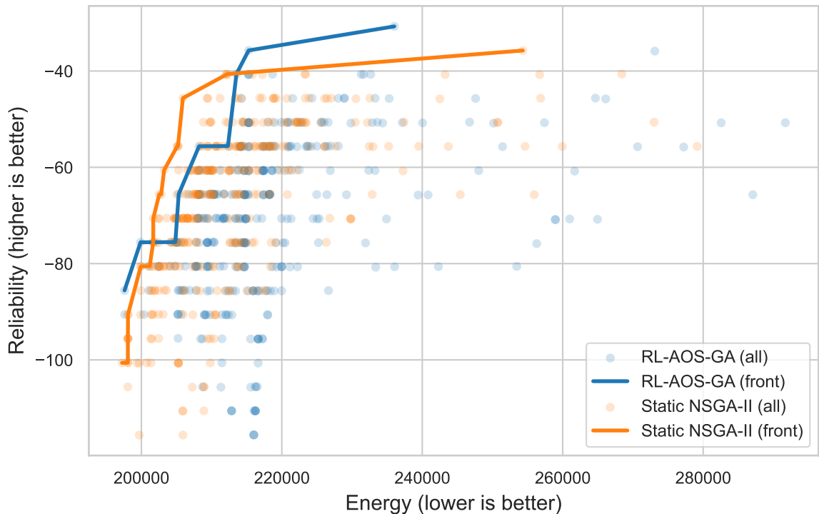
Pareto Trade-off (Energy vs Reliability)
