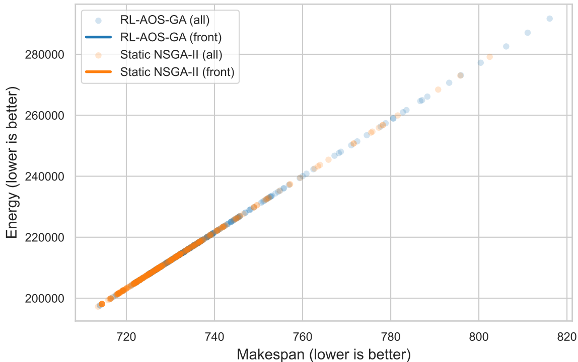
Pareto Trade-off (Makespan vs Energy)
